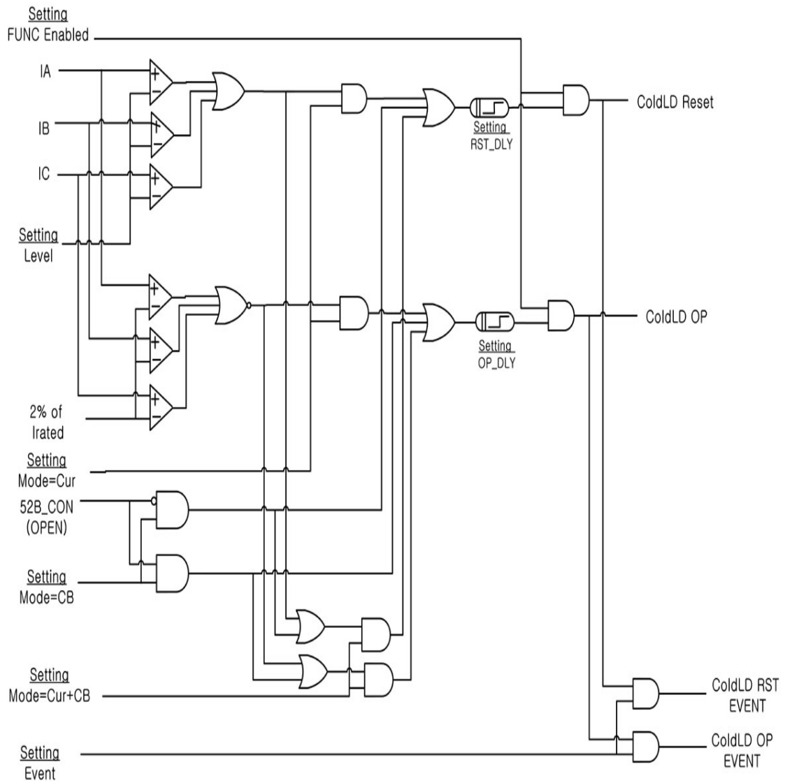
<Figure 8. Cold Load Pick-Up 요소 Logic Diagram>
