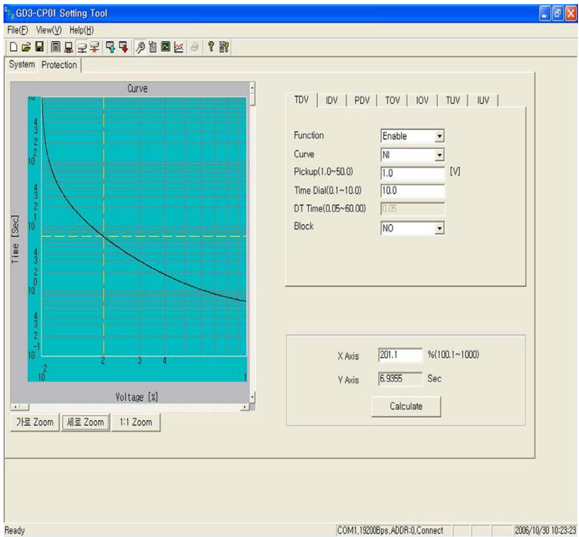
<Figure 18. GD3-CP01 Protection Setting>
