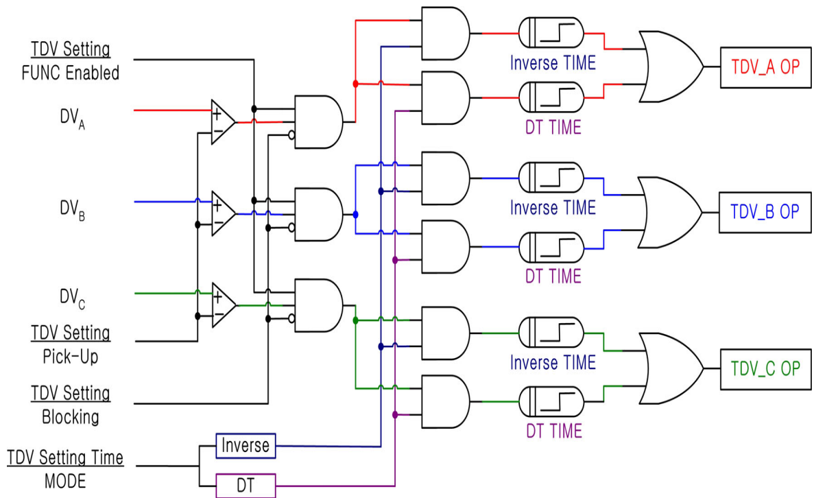
<Figure 1. TDV Logic Diagram>
