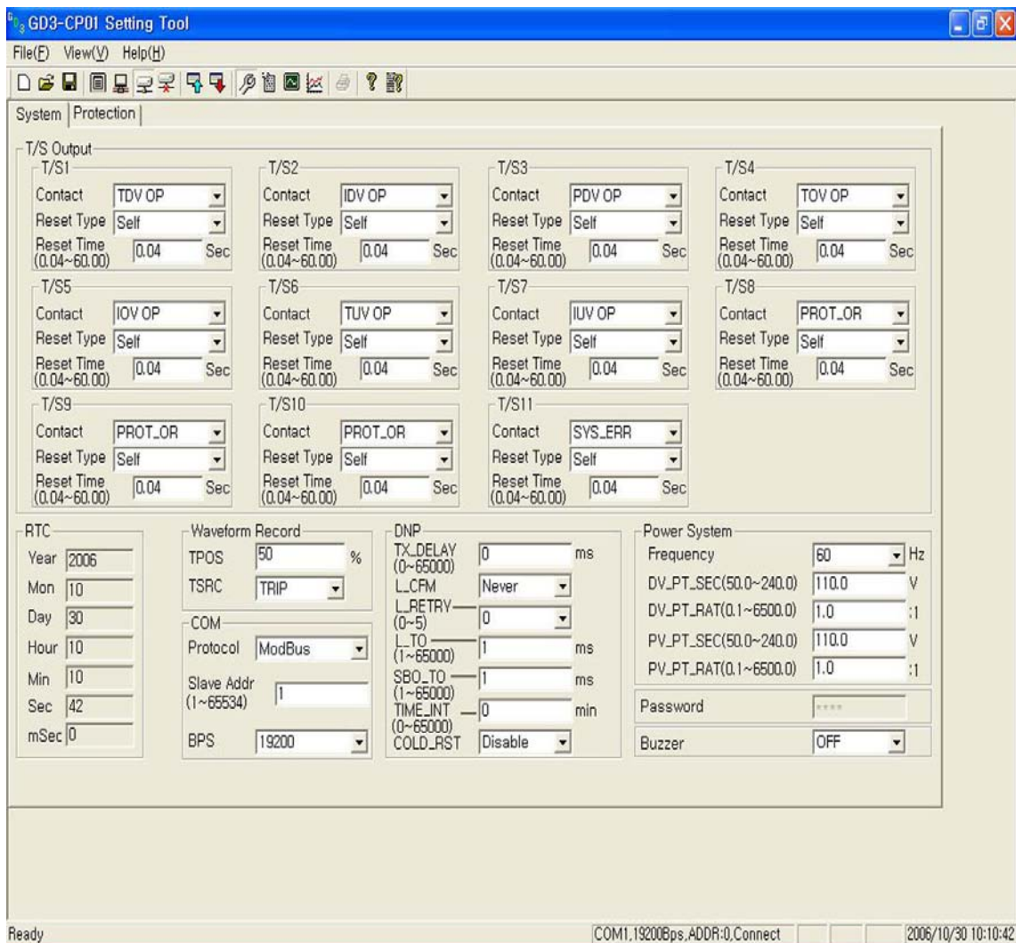
<Figure 17. GD3-CP01 System Configuration>
