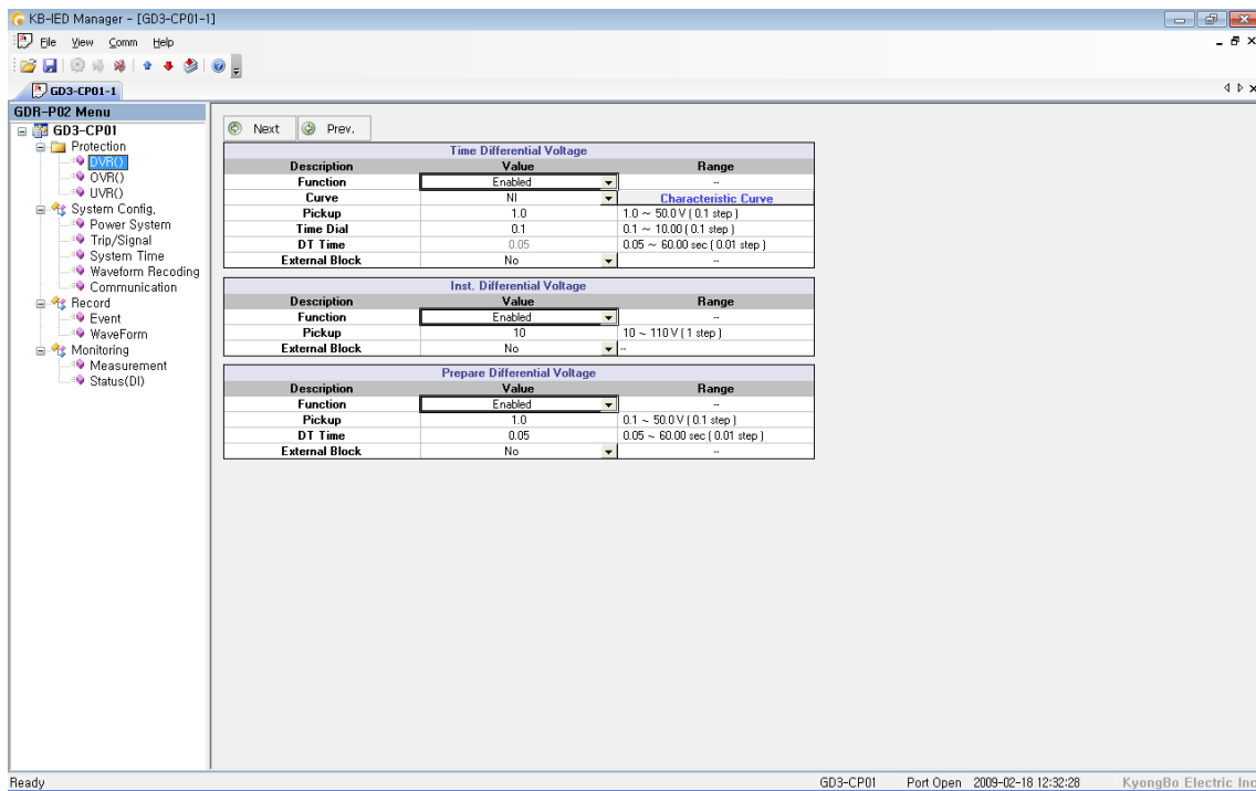
<Figure 13. GD3-CP01 Protection Setting>
