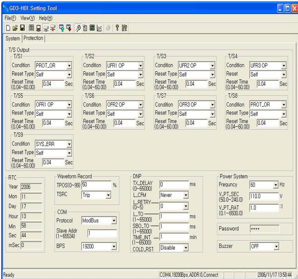
<Figure 10. GD3-H01 System Configuration>
