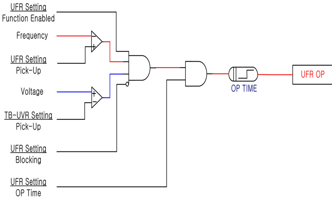
<Figure 2. UFR Logic Diagram>
