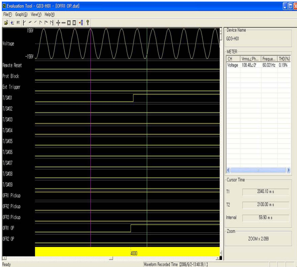
<Figure 15. GD3-H01 Evaluation Tool>
