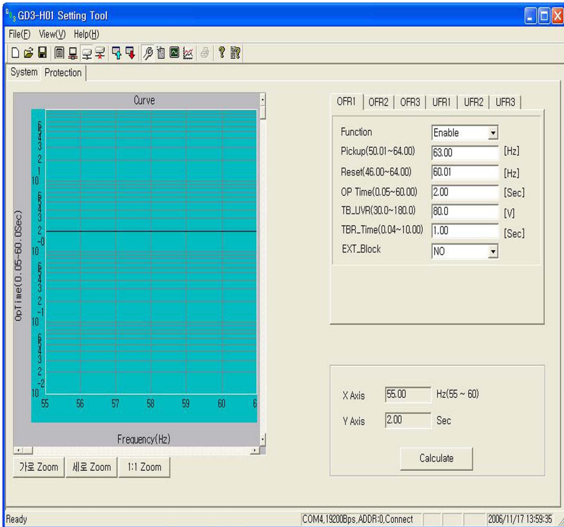
<Figure 11. GD3-H01 Protection Setting>
