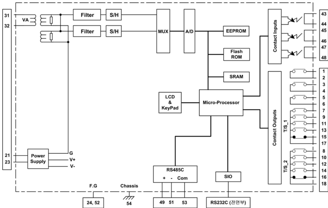
<부도 2. Relay Hardware Internal Structure>
