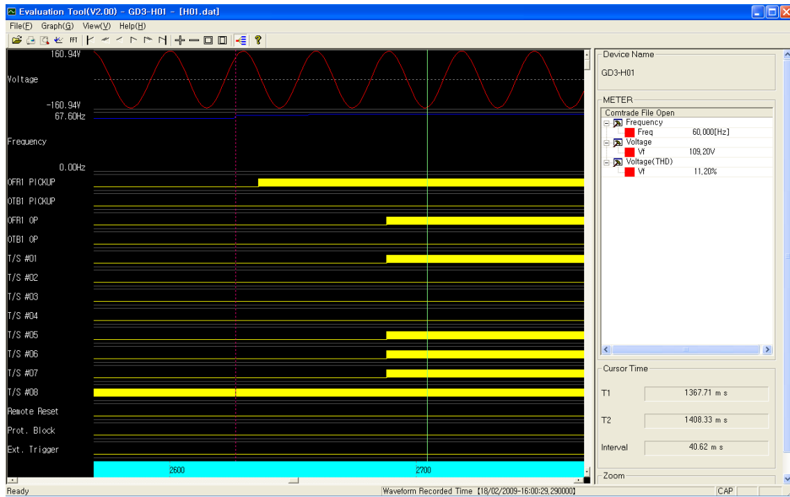
<Figure 18. GD3-H01 Evaluation Tool>
