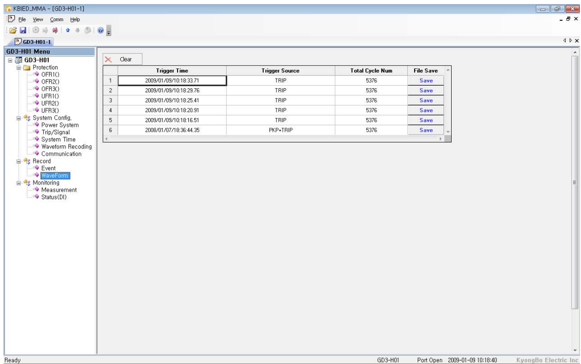
<Figure 15. GD3-H01 Waveform>
