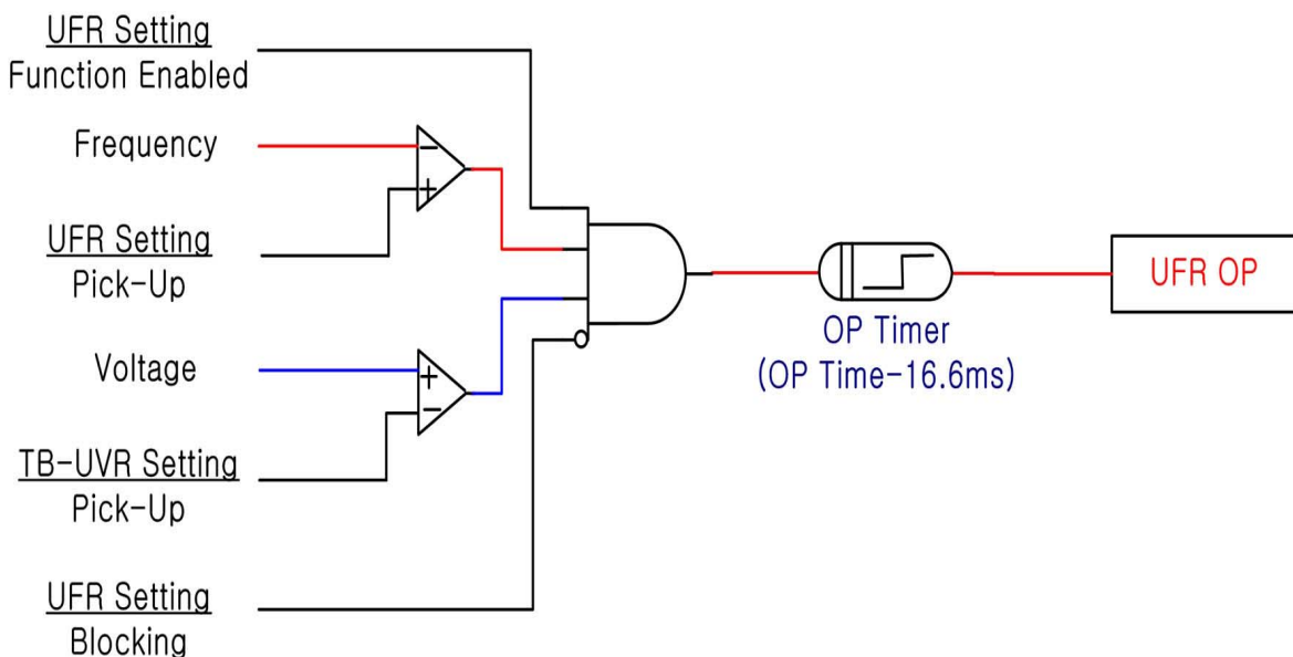
<Figure 2. UFR Logic Diagram>
