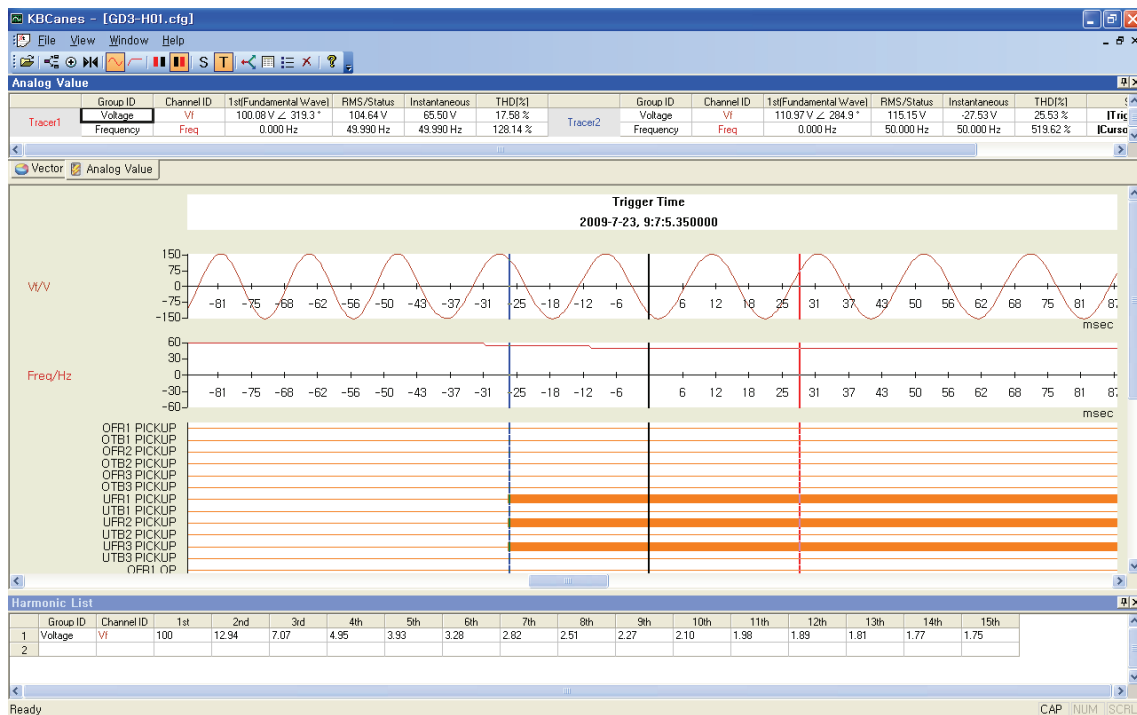
<Figure 18. KBcanes>
