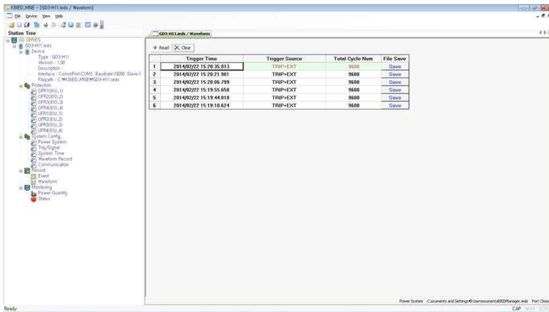
<Figure 24. WaveForm>
