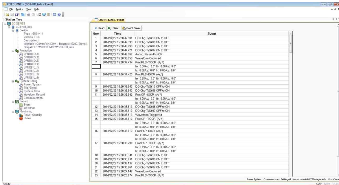
<Figure 23. Event>
