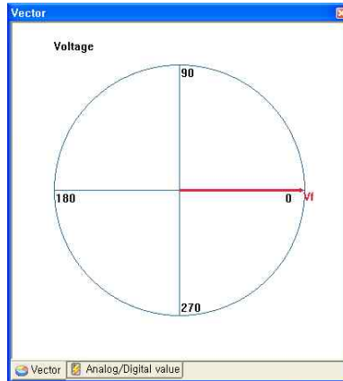
<Figure 31. Vector>
