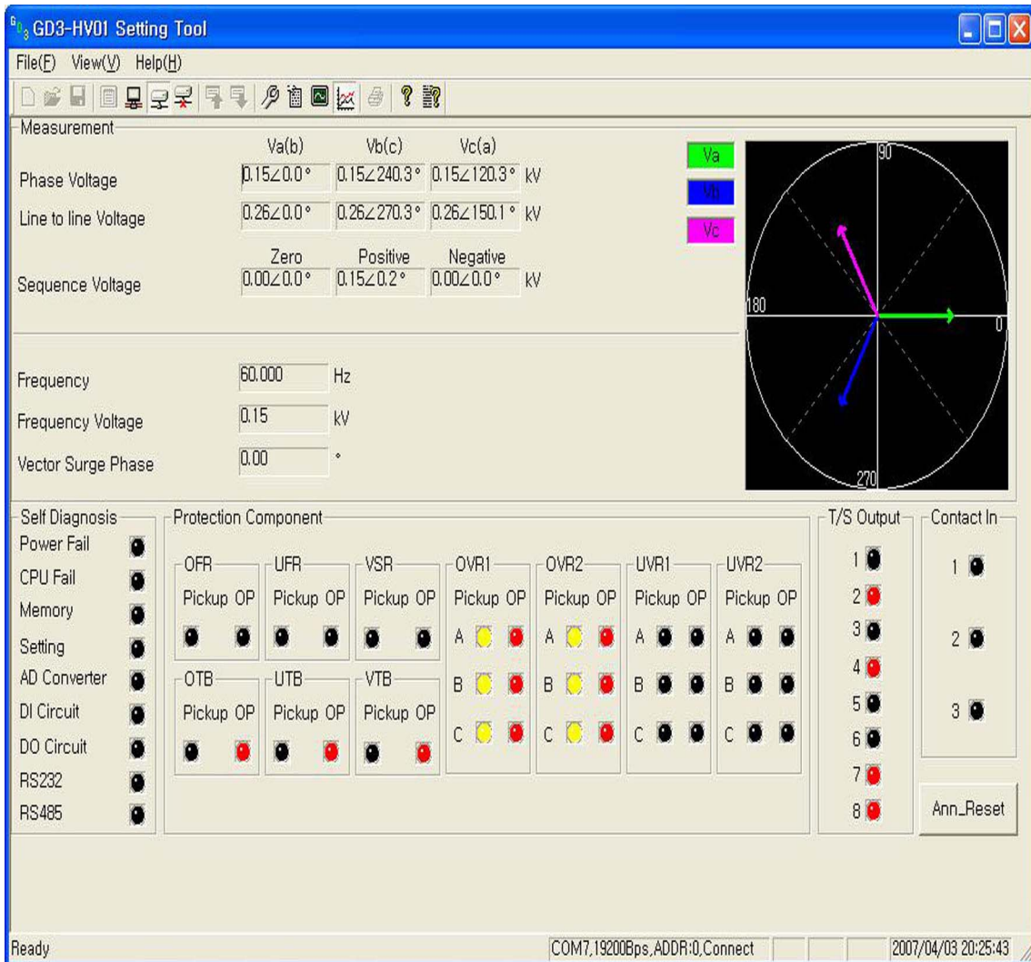
<Figure 20. GD3-HV01 Monitor>
