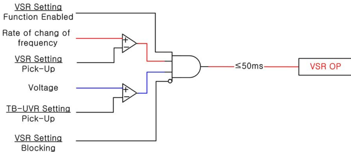
<Figure 6. VSR Logic Diagram>
