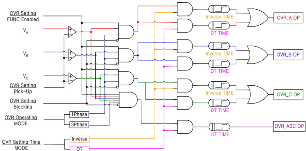
<Figure 3. OVR Logic Diagram>
