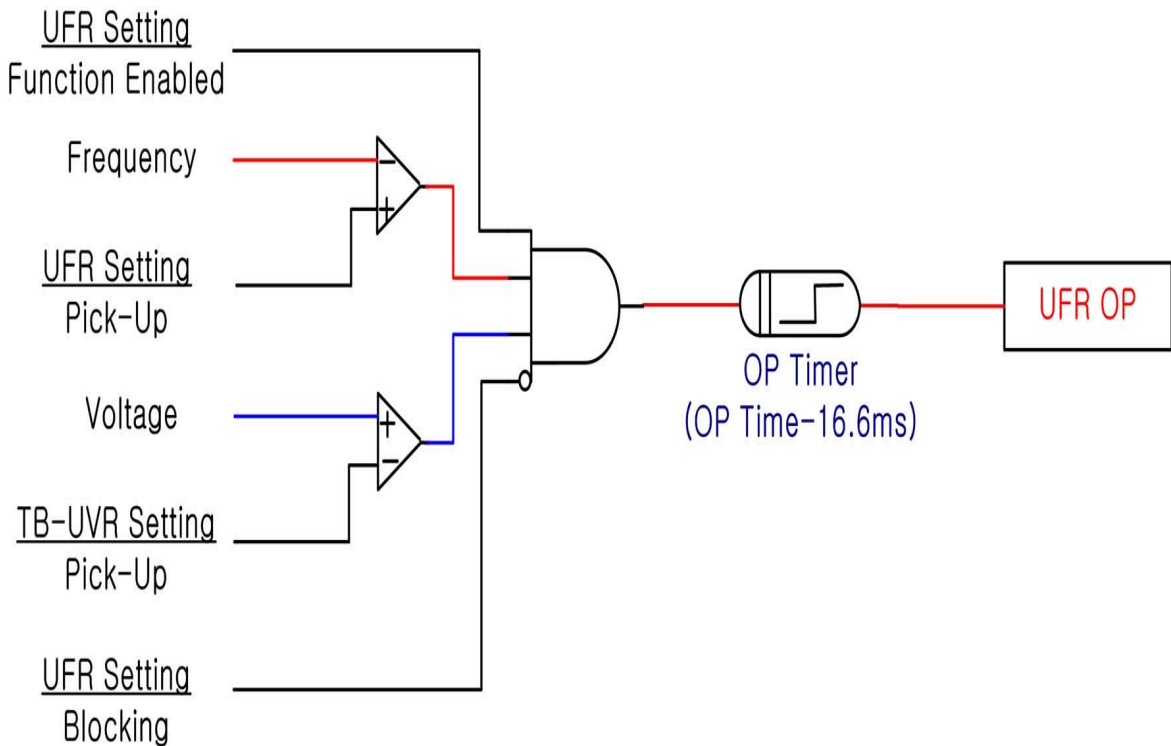
<Figure 2. UFR Logic Diagram>
