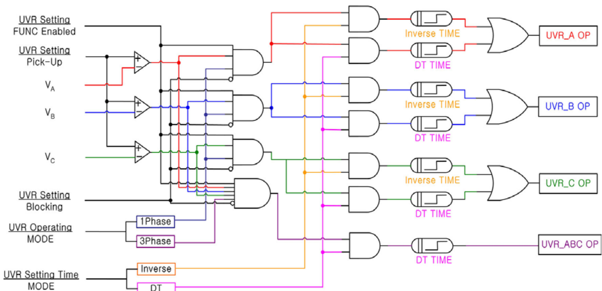
<Figure 4. UVR Logic Diagram>
