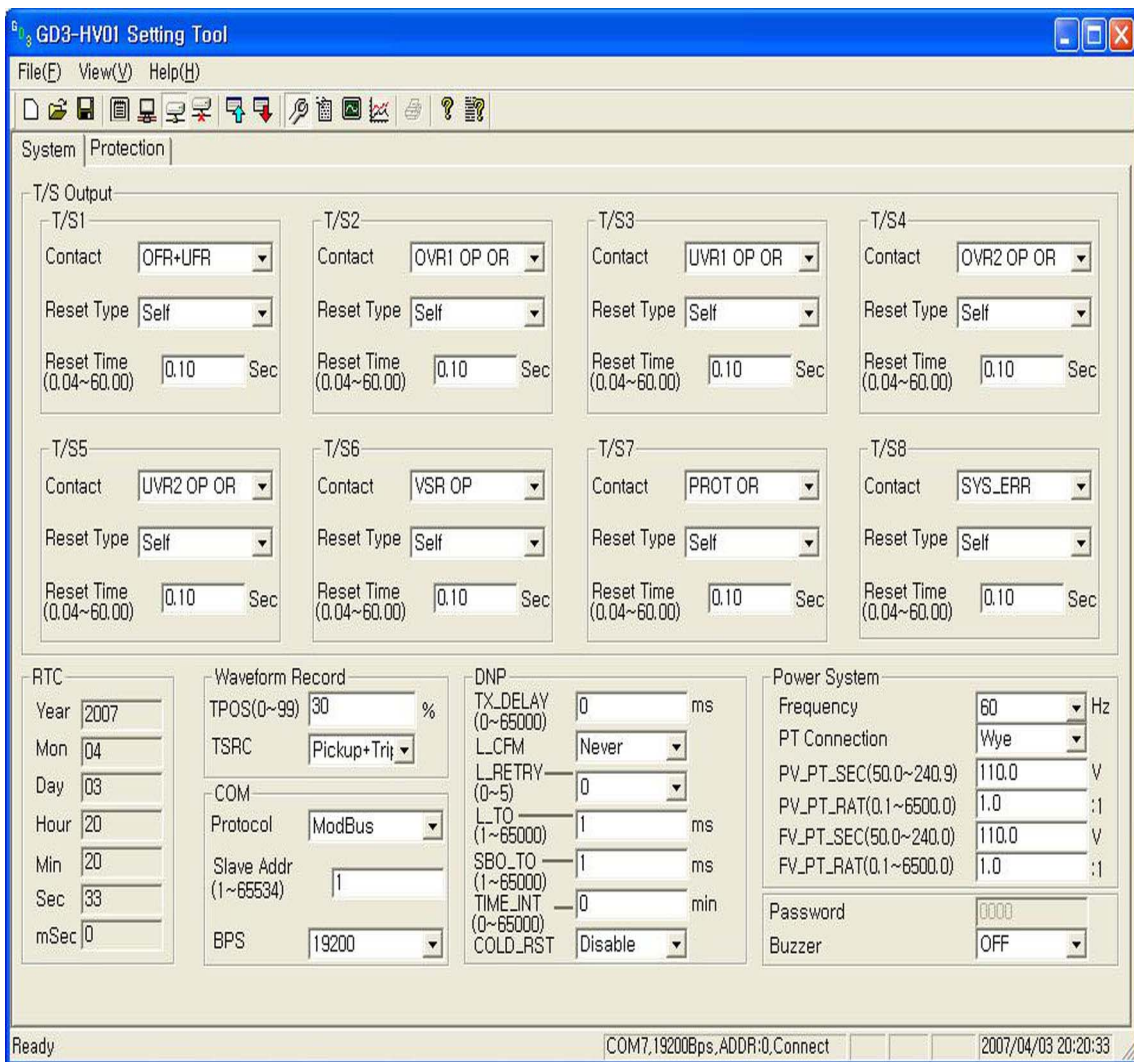
<Figure 16. GD3-HV01 System Configuration>
