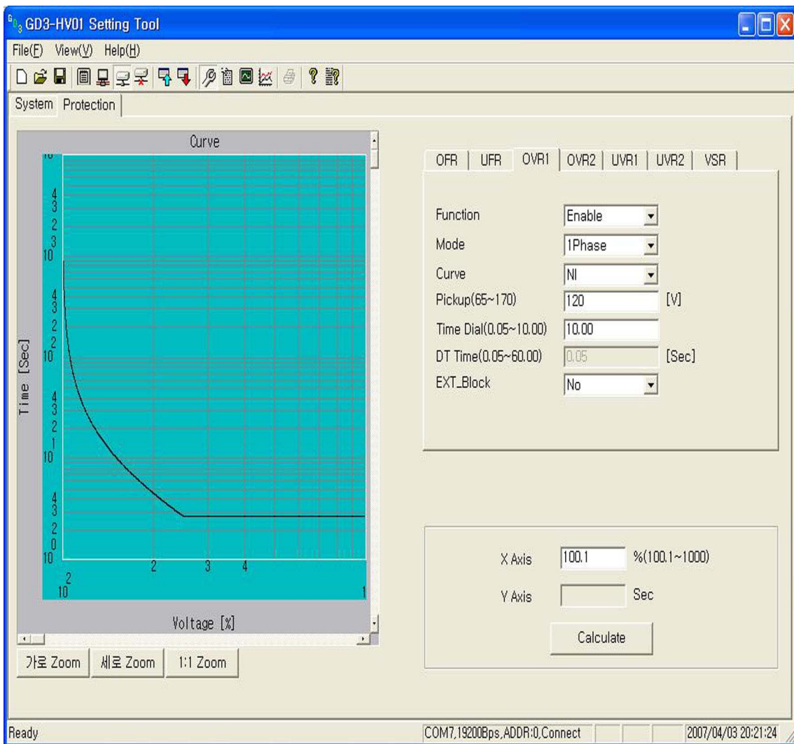
<Figure 17. GD3-HV01 Protection Setting>
