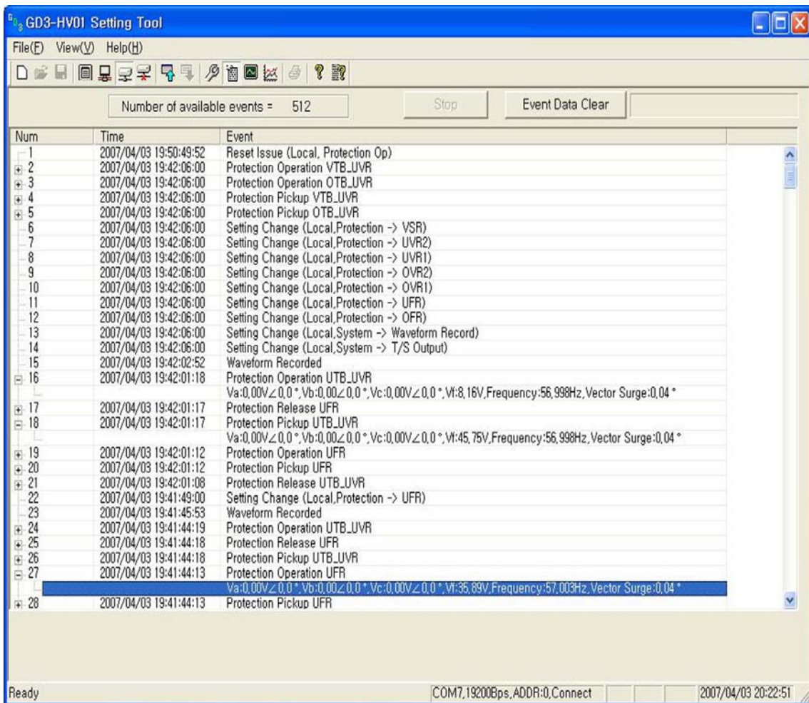
<Figure 18. GD3-HV01 Event>
