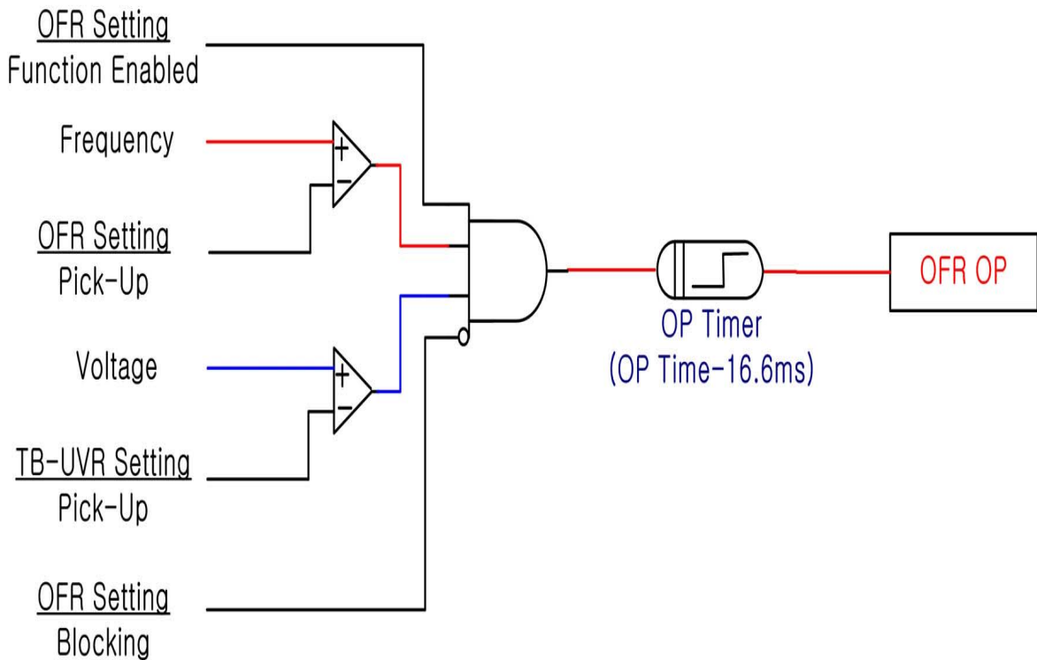
<Figure 1. OFR Logic Diagram>
