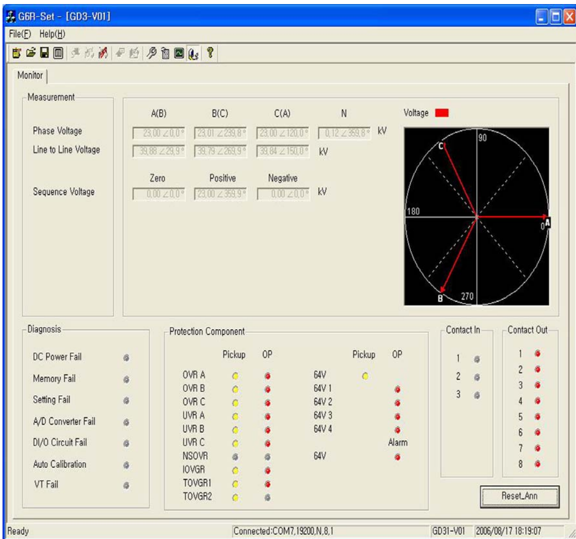
<Figure 19. GD3-V01 Monitor>
