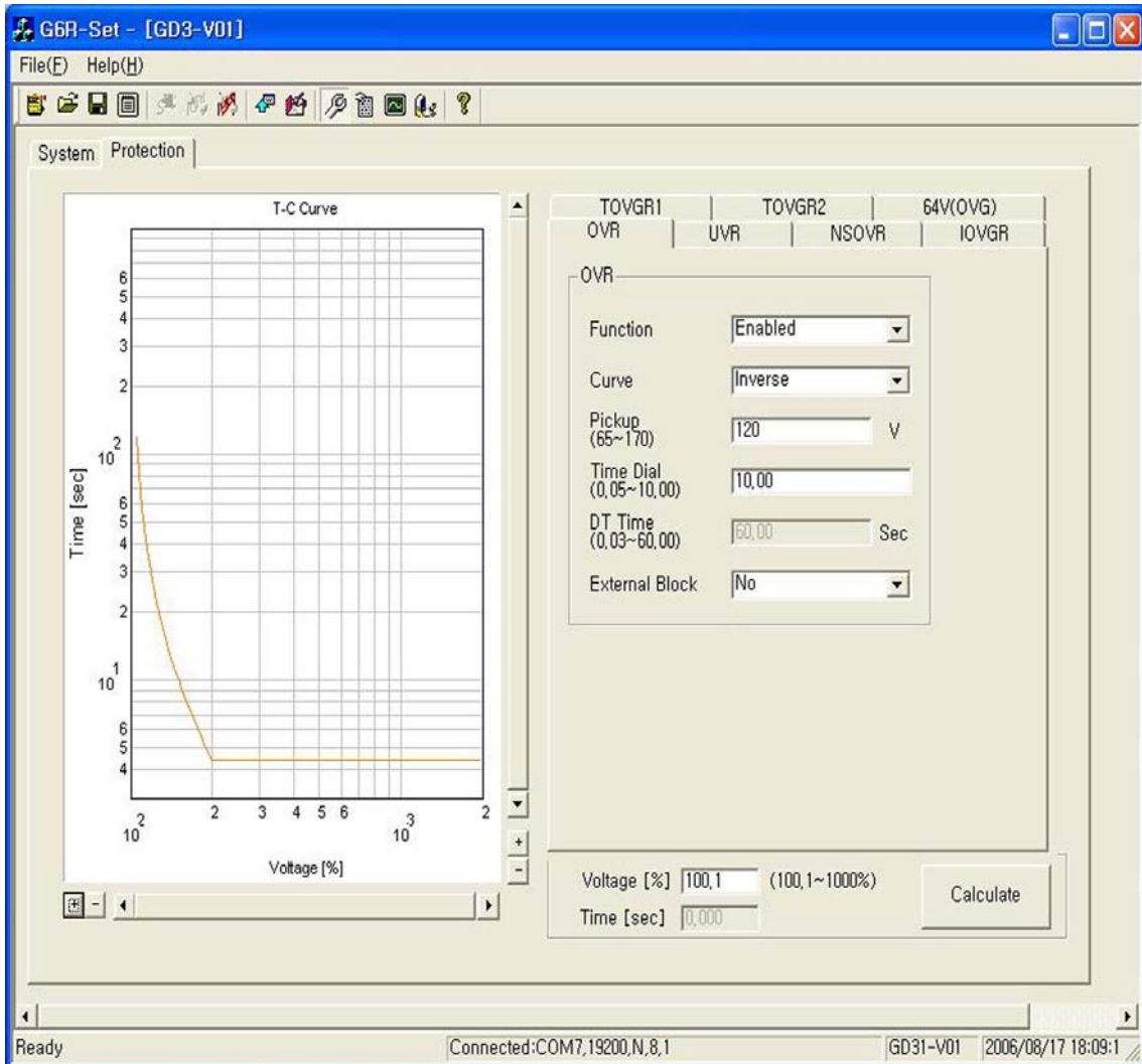
<Figure 16. GD3-V01 Protection Setting>
