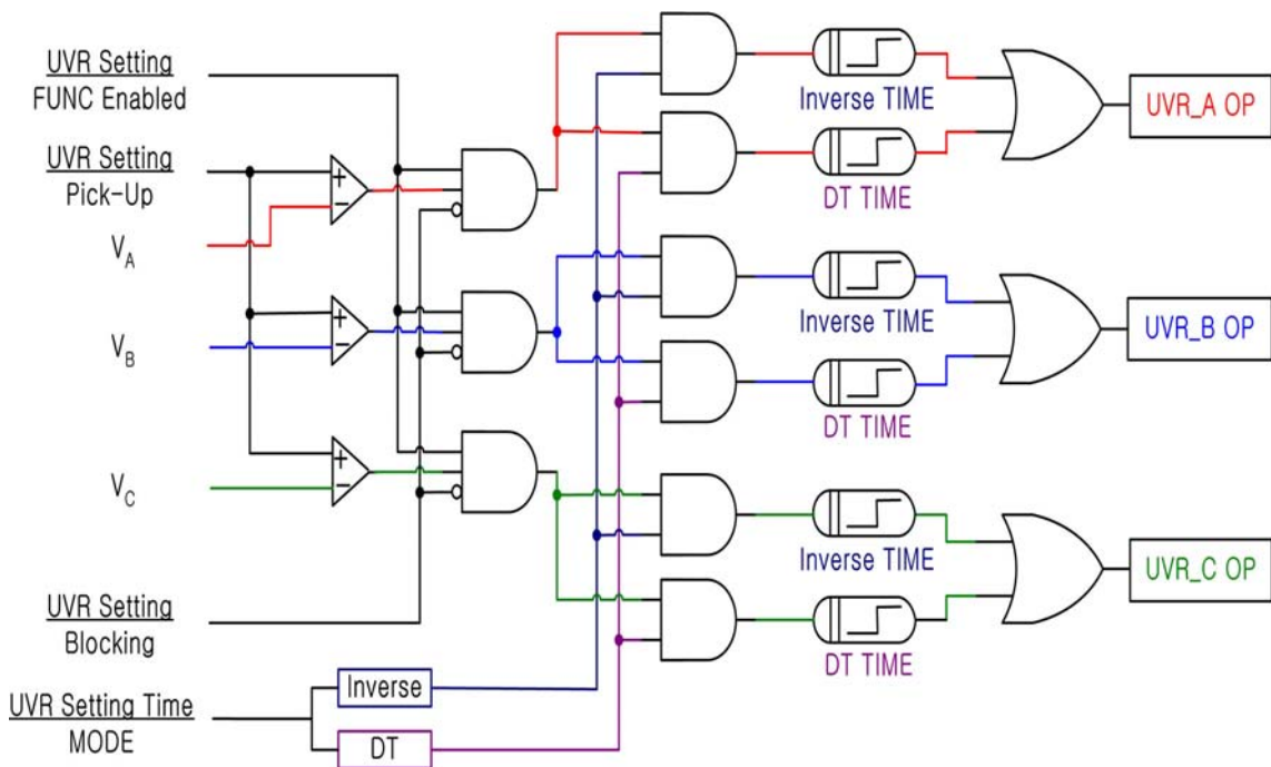
<Figure 2. UVR Logic Diagram>
