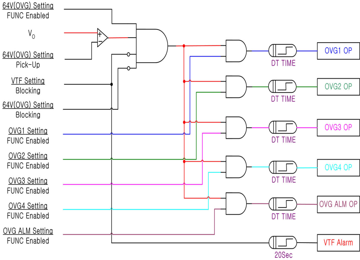
<Figure 6. 64V(OVG) Logic Diagram>
