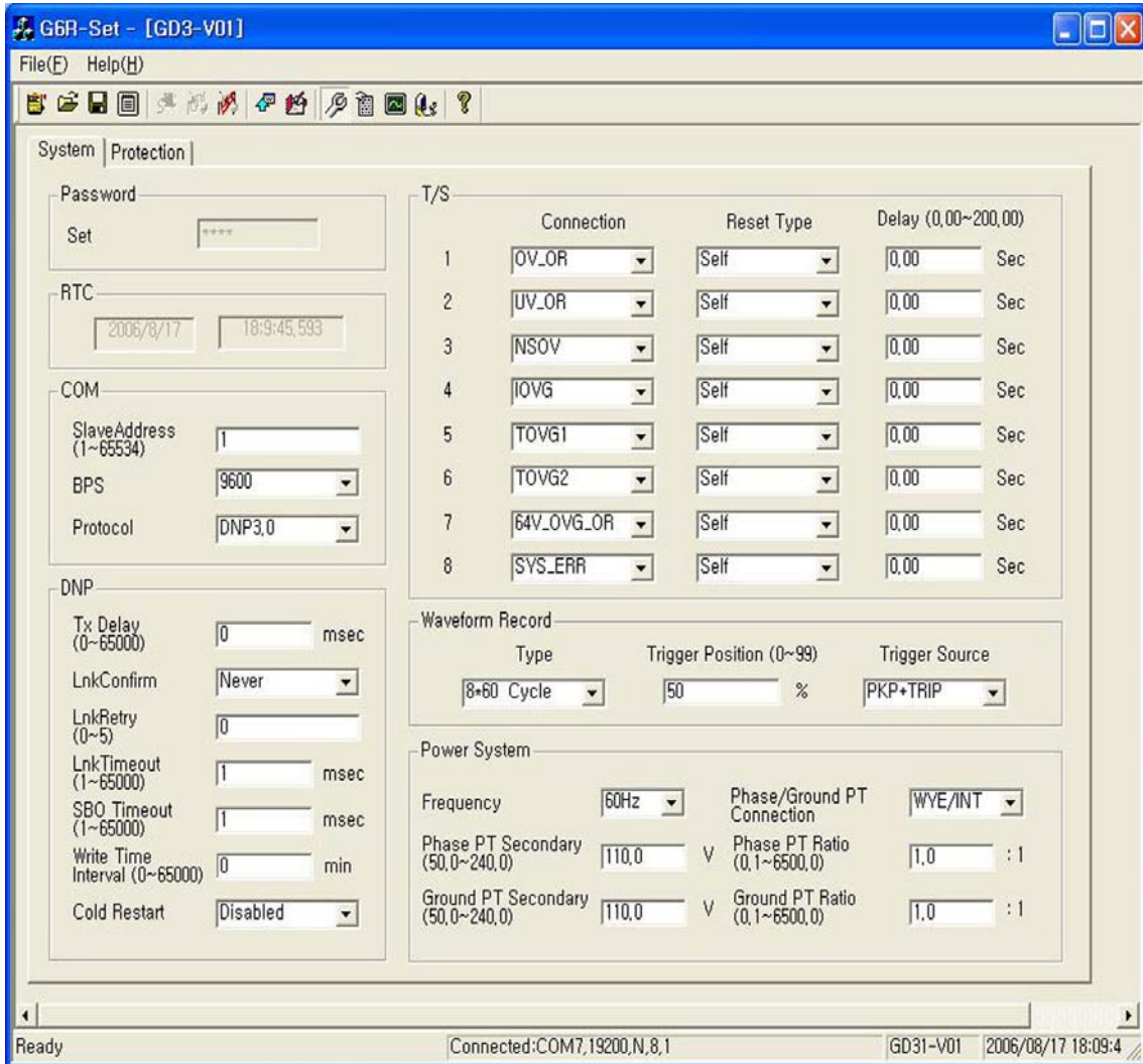
<Figure 15. GD3-V01 System Configuration>
