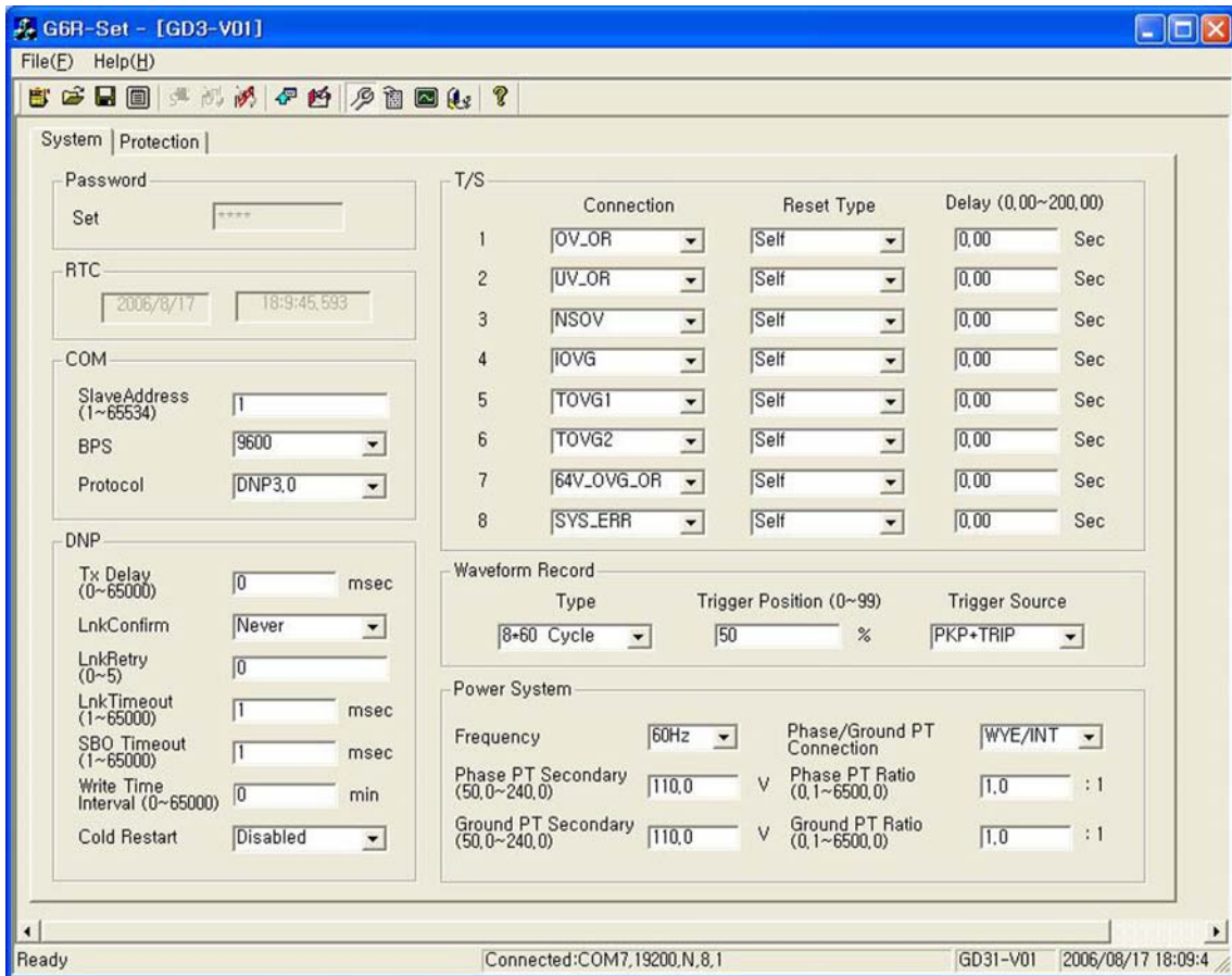
<Figure 17. GD3-V01 System Configuration>
