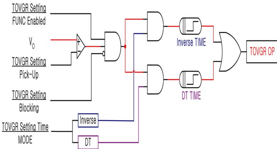
<Figure 5. TOVGR Logic Diagram>
