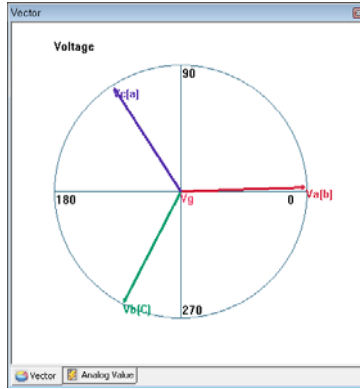
<Figure 35. Vector>
