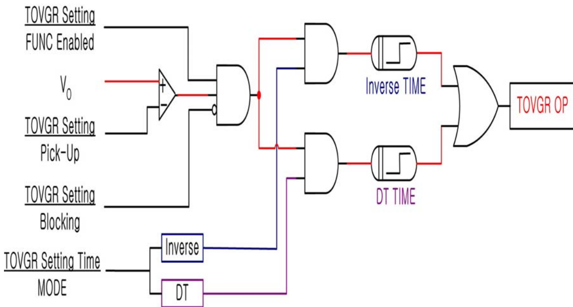
<Figure 5. TOVGR Logic Diagram>
