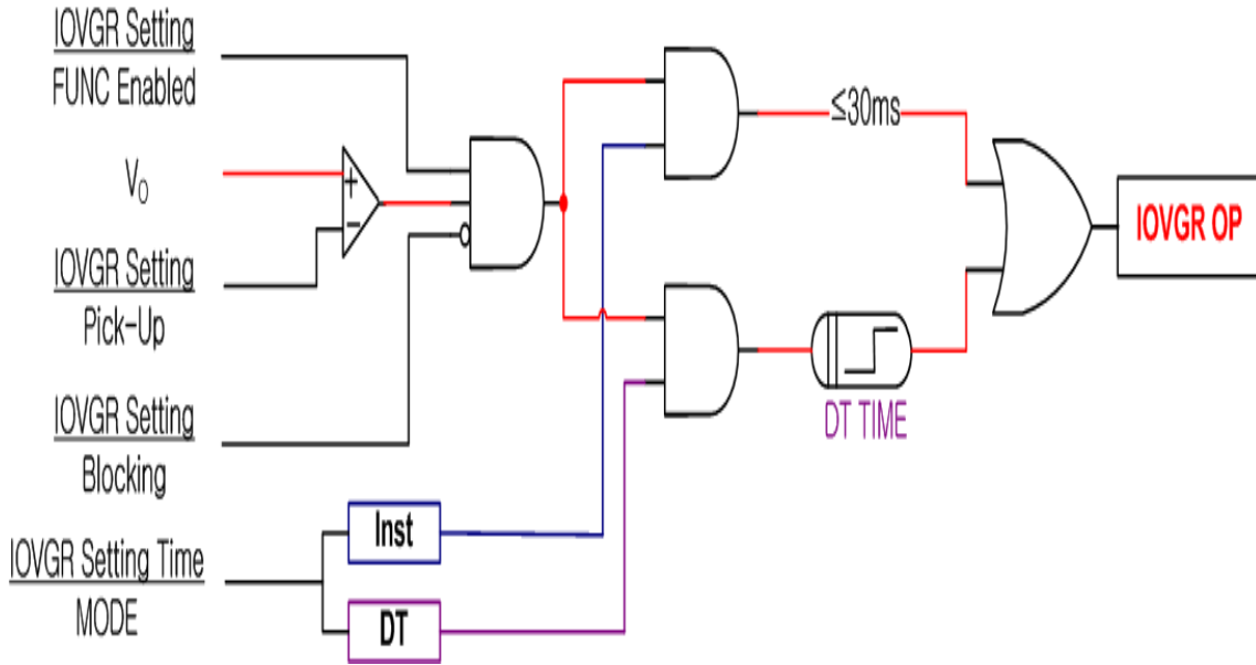
<Figure 4. IOVGR Logic Diagram>
