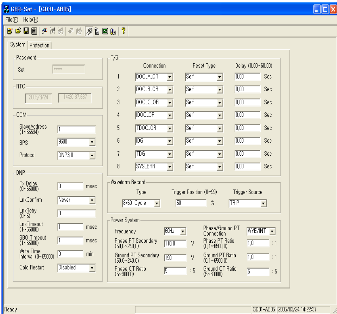
<Figure 16. GD31-AB05 System Configuration>
