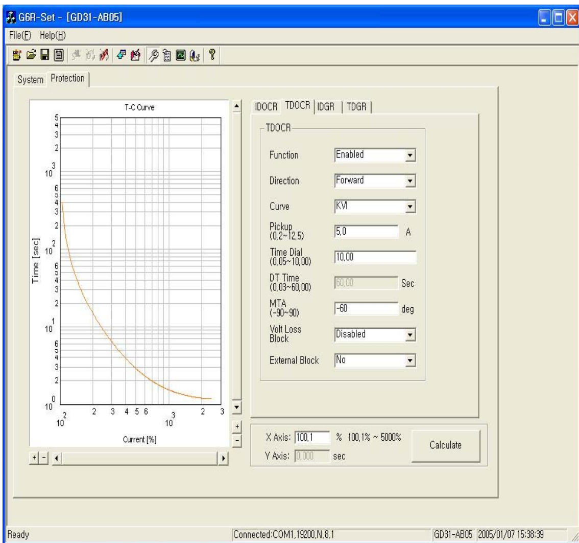
<Figure 17. GD31-AB05 Protection Setting>
