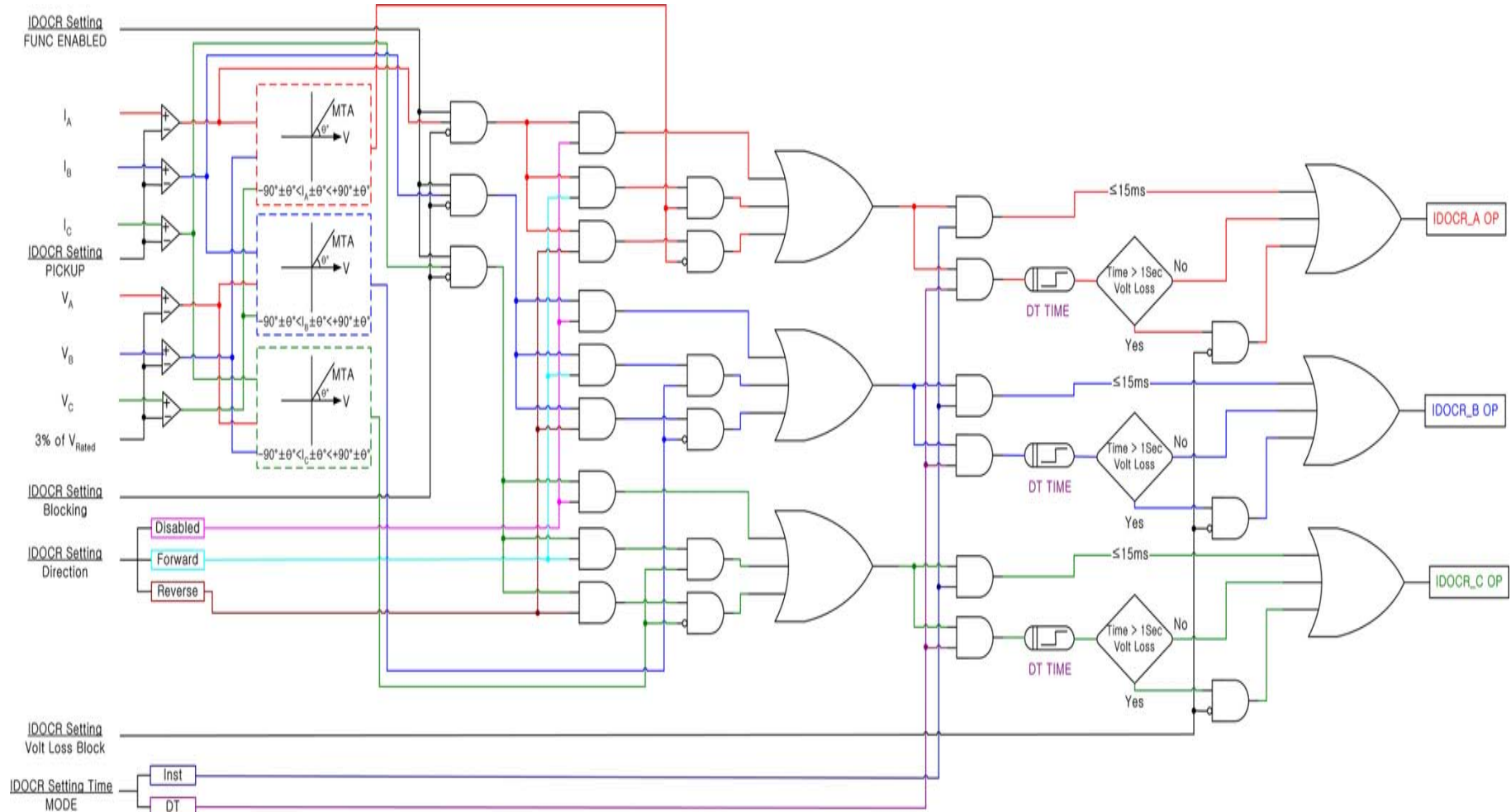
<Figure 3. IDOCR Logic Diagram>
