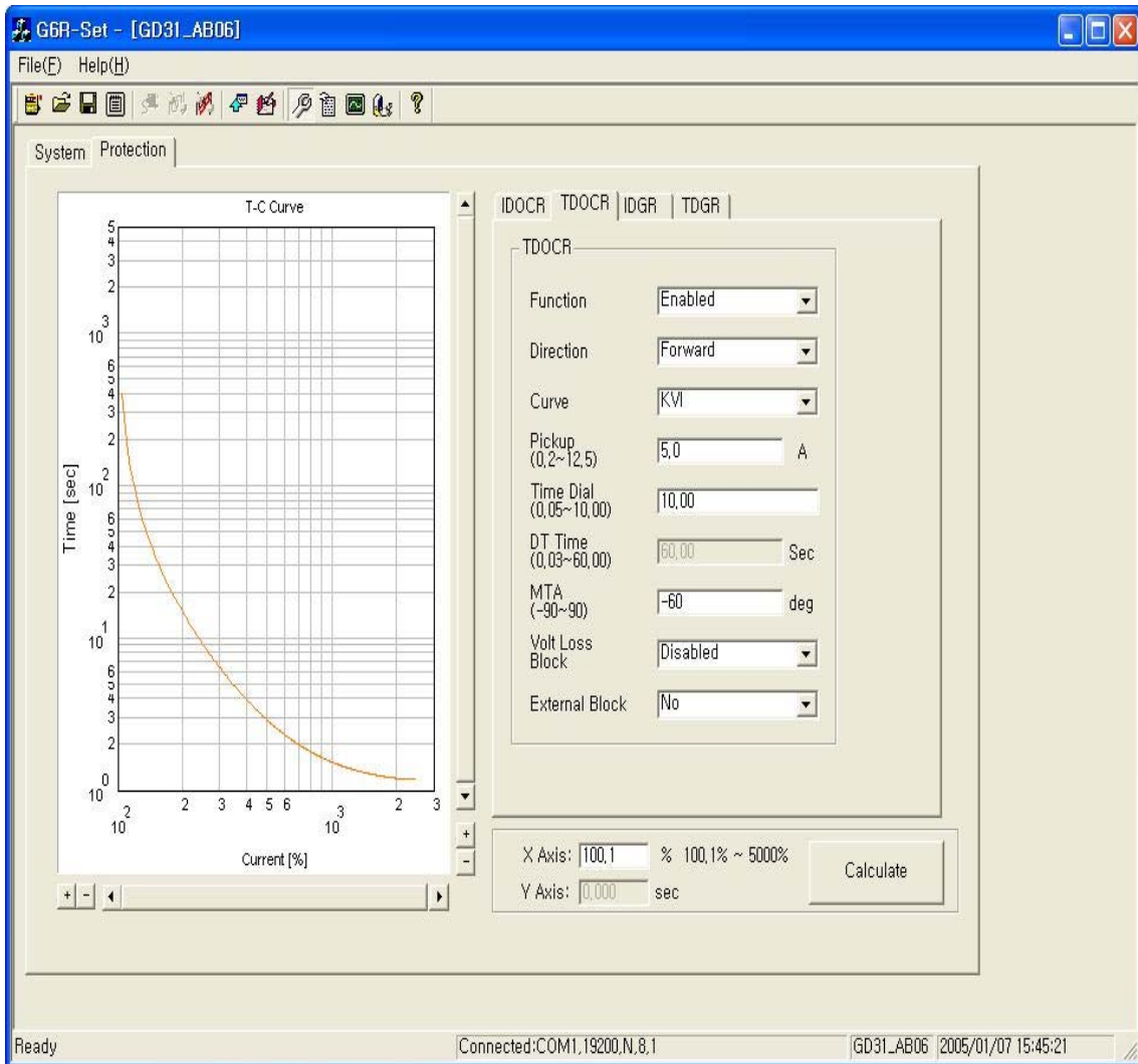
<Figure 14. GD31-AB06 Protection Setting>
