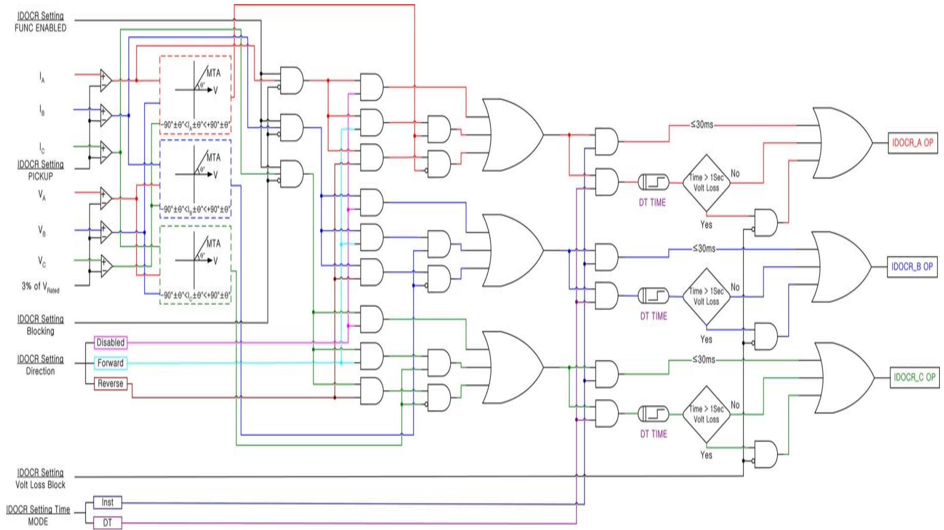
<Figure 3. IDOCR Logic Diagram>
