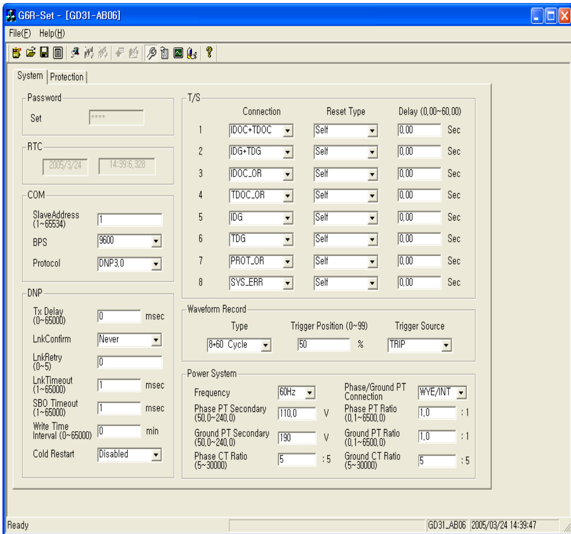
<Figure 13. GD31-AB06 System Configuration>
