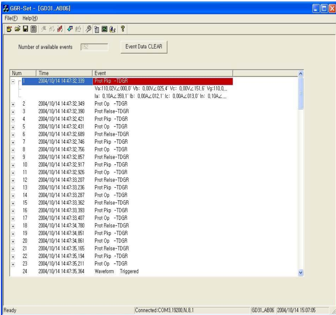
<Figure 15. GD31-AB06 Event>
