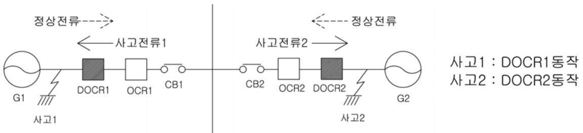
<Figure 1. IDOCR Logic Diagram>
