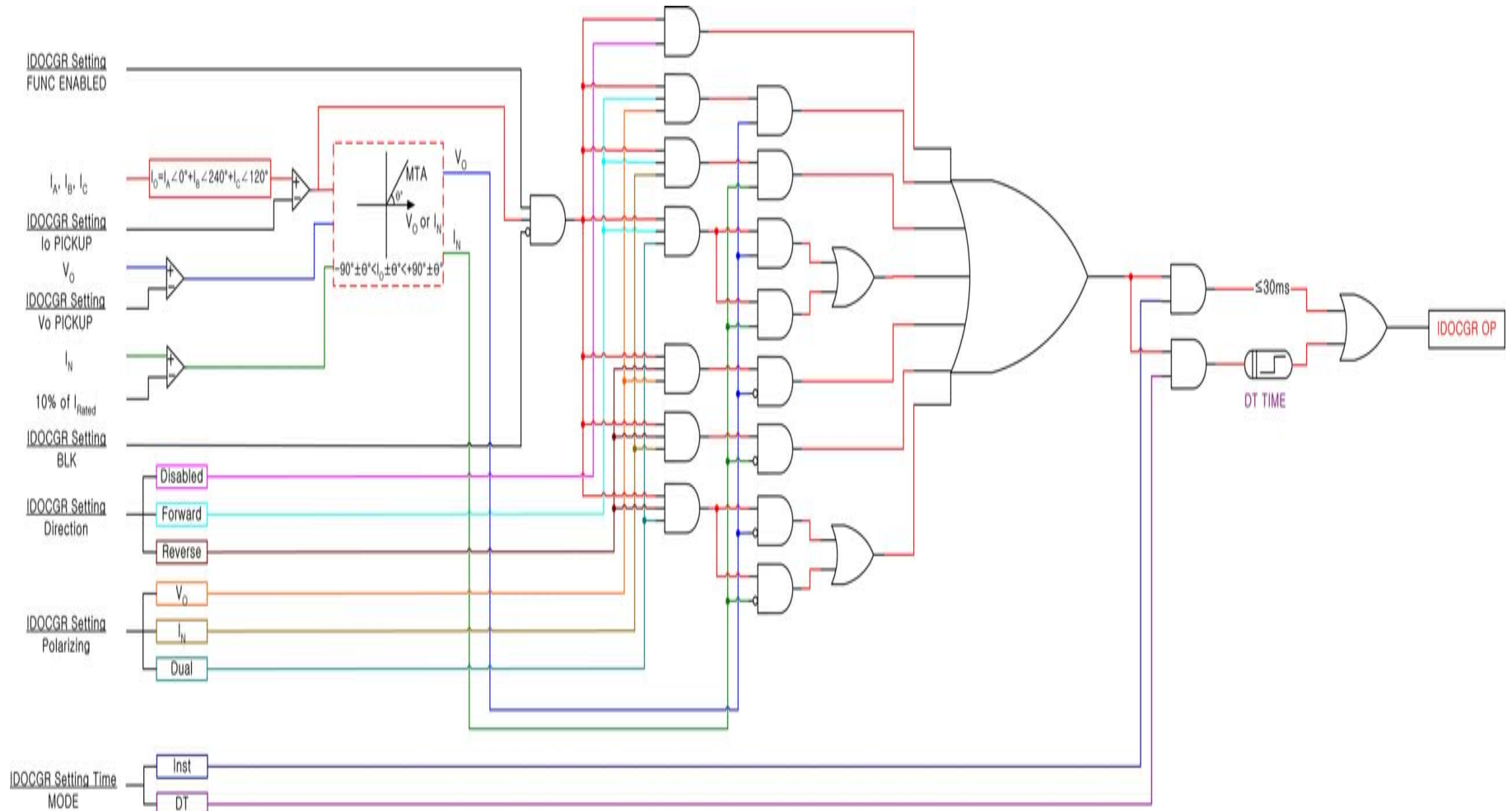
<Figure 6. IDGR Logic Diagram>
