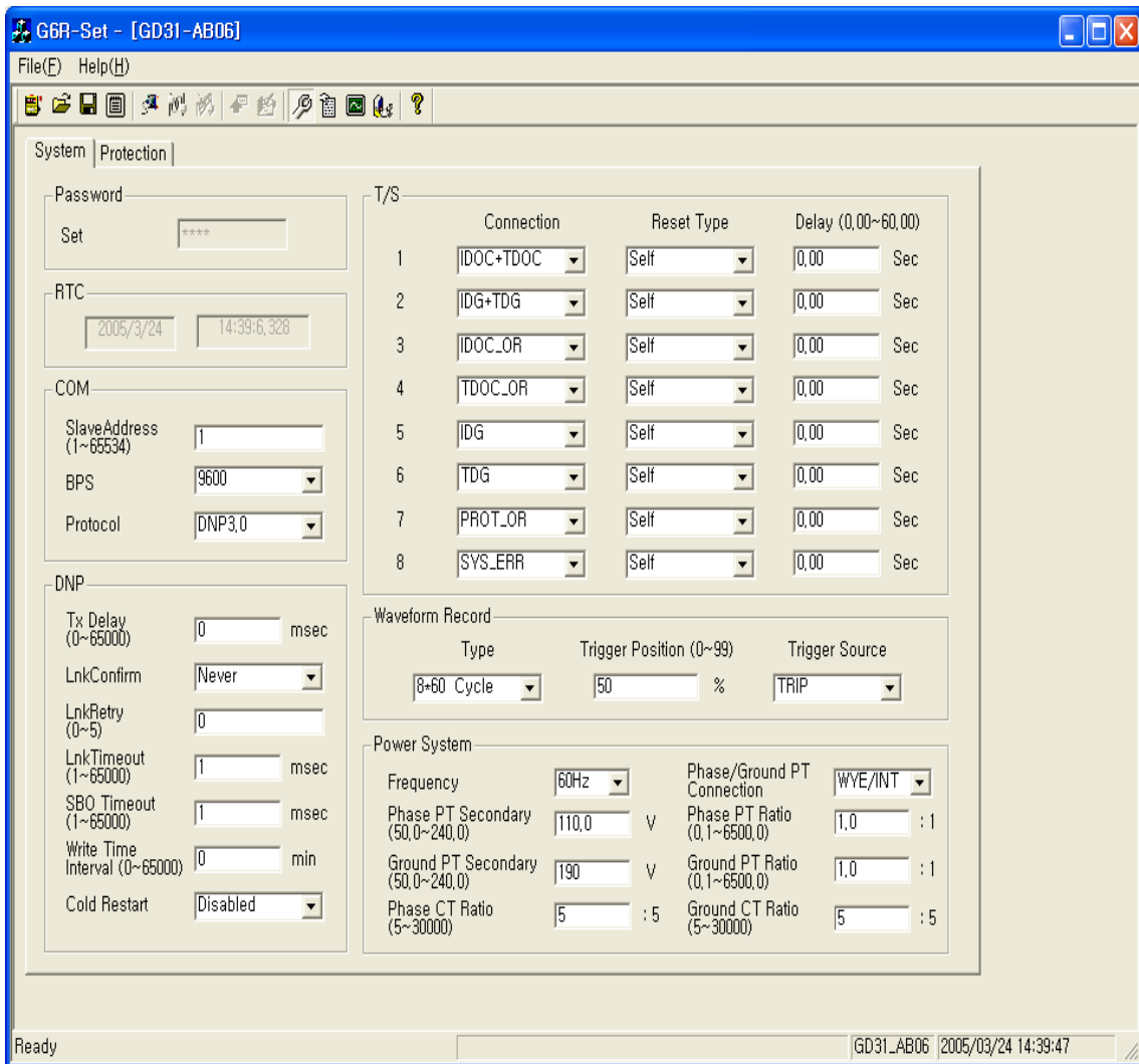
<Figure 16. GD31-AB06 System Configuration>
