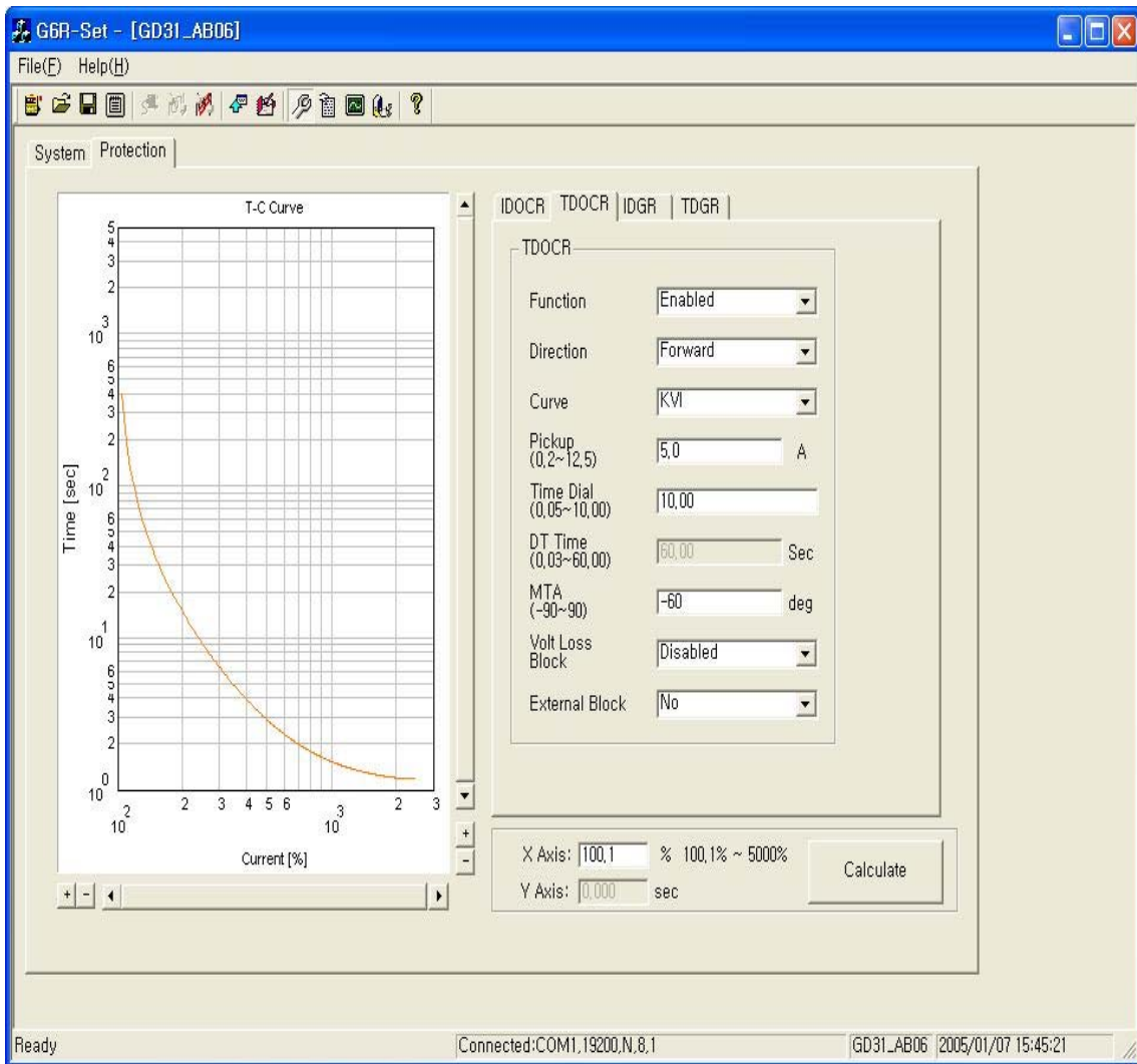
<Figure 17. GD31-AB06 Protection Setting>
