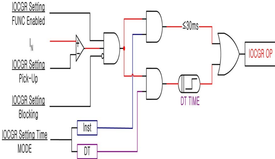
<Figure 3. IOCGR Logic Diagram>
