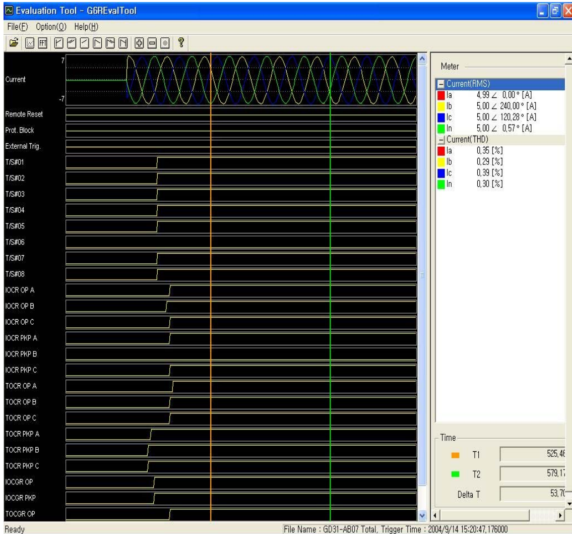
<Figure 15. GD31-AB07 Fault Evaluation Tool>
