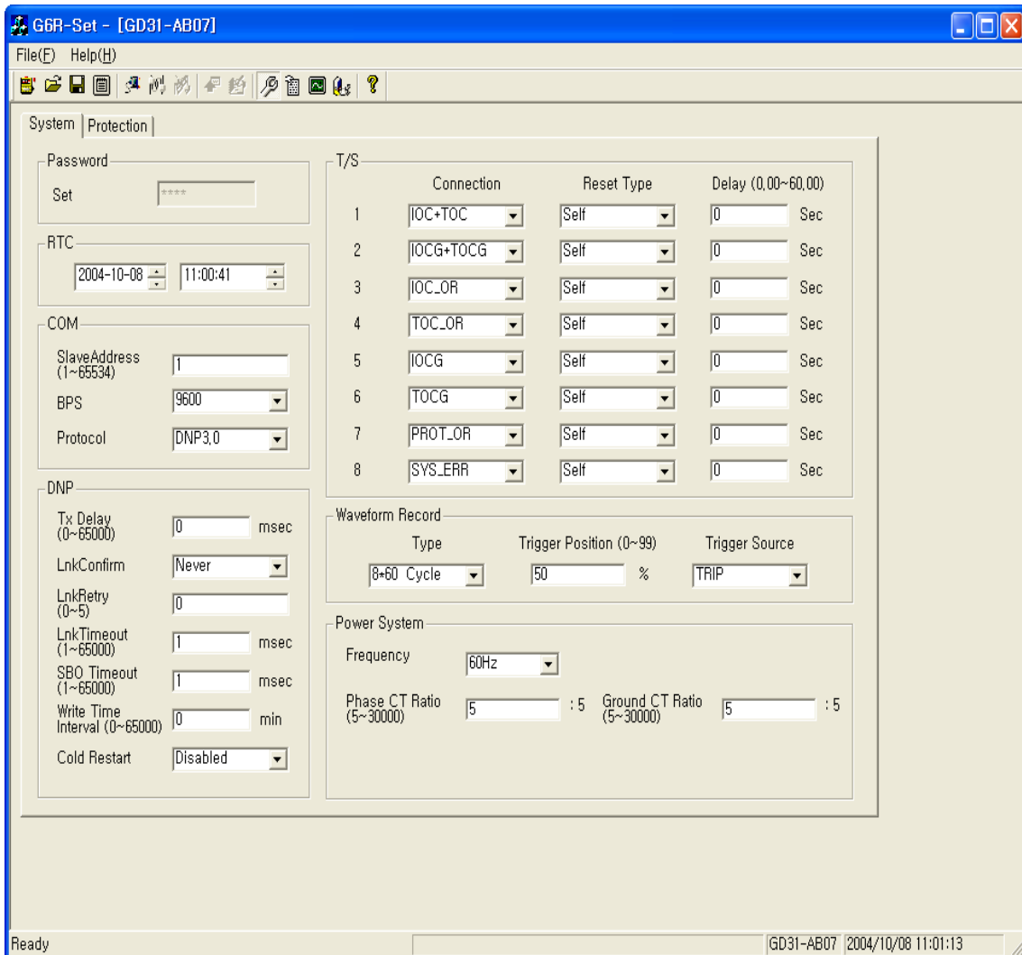
<Figure 10. GD31-AB07 System Configuration>
