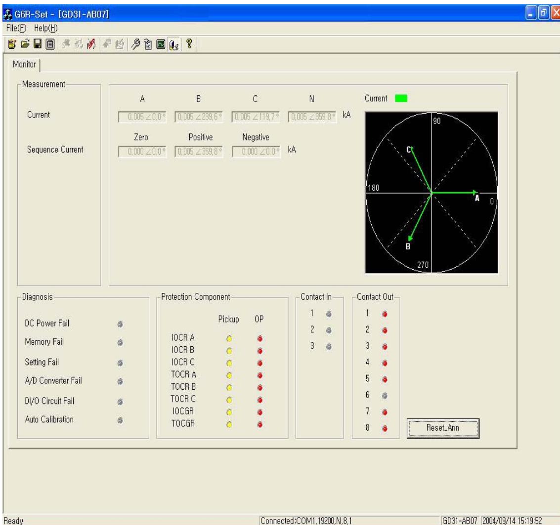
<Figure 14. GD31-AB07 Monitor>
