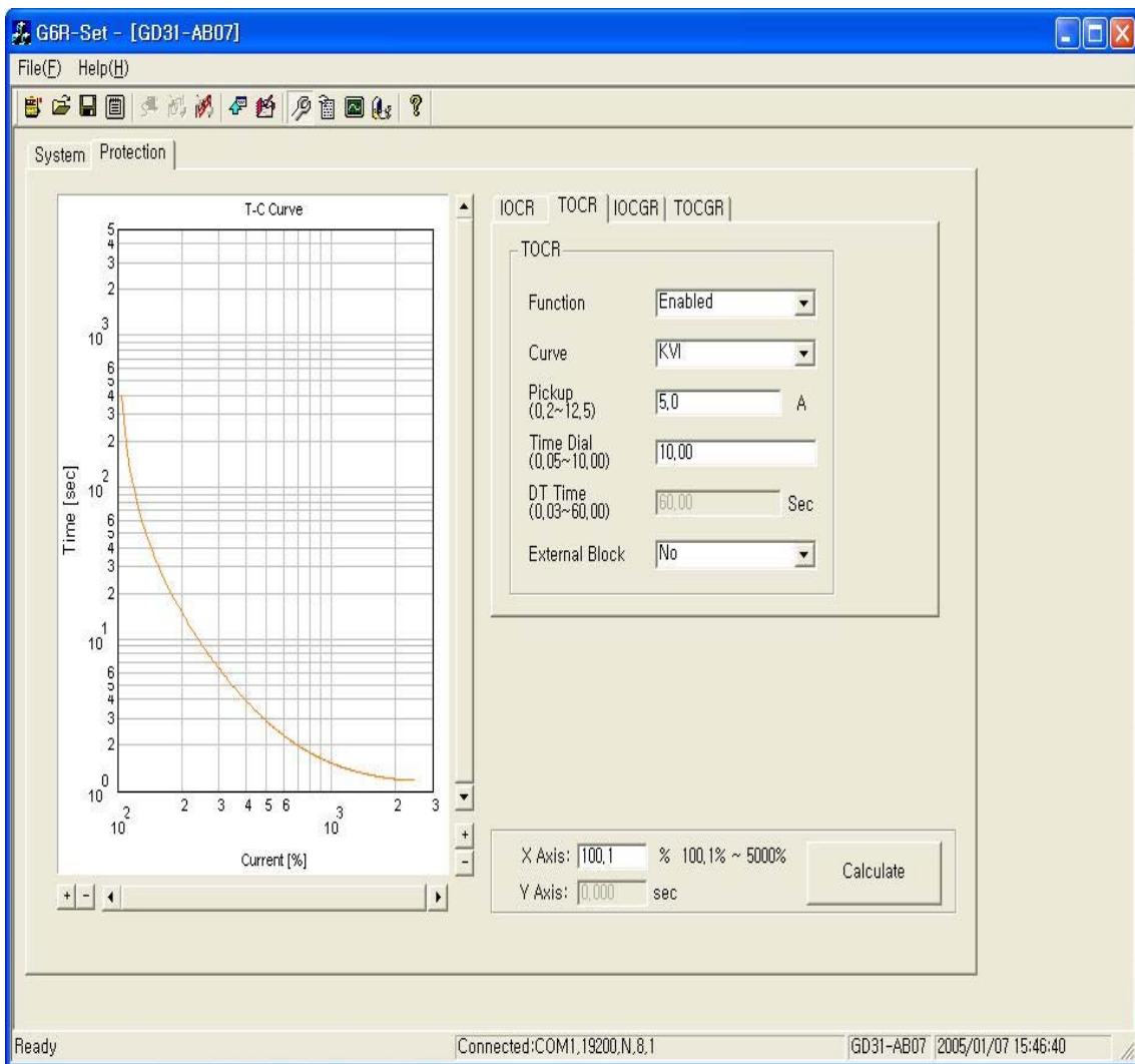
<Figure 11. GD31-AB07 Protection Setting>
