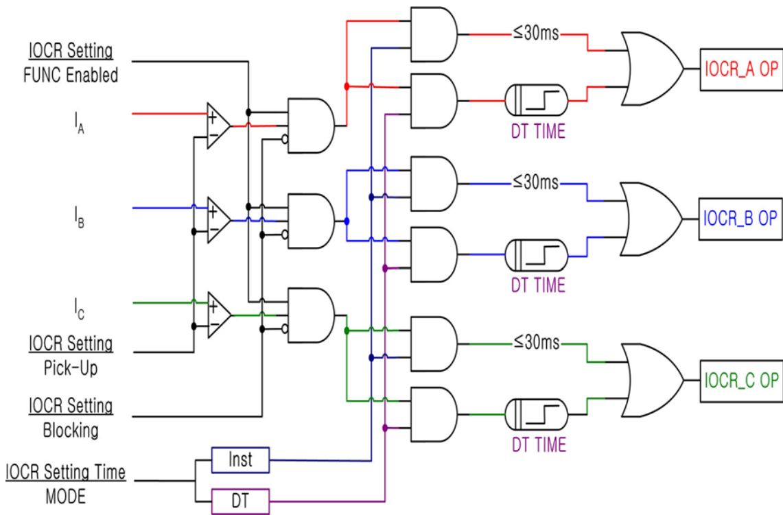
<Figure 1. IOCR Logic Diagram>
