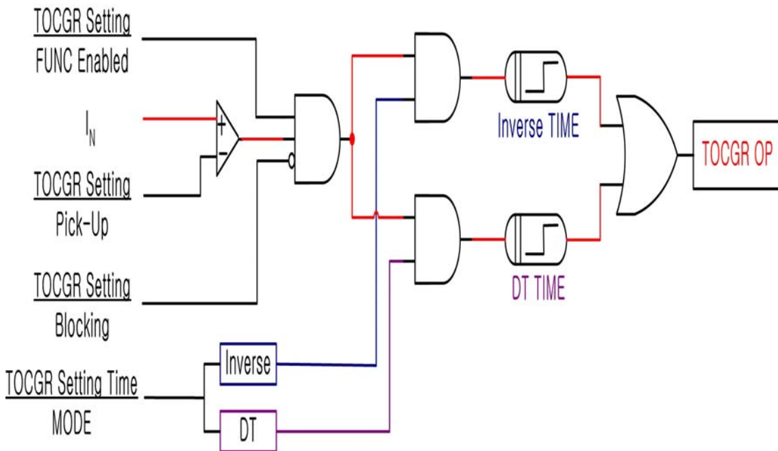
<Figure 4. TOCGR Logic Diagram>
