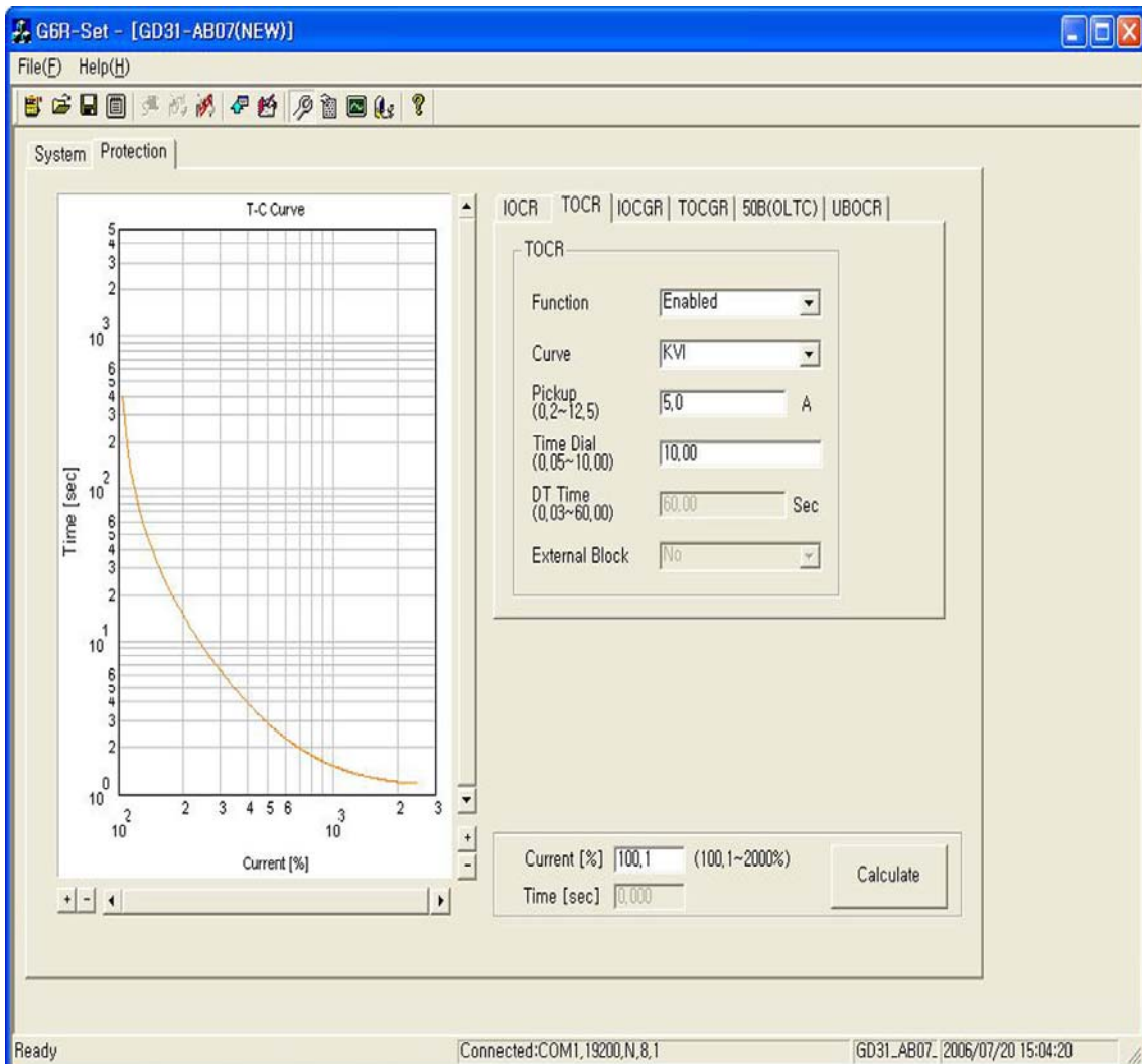
<Figure 15. GD31-AB07 Protection Setting>
