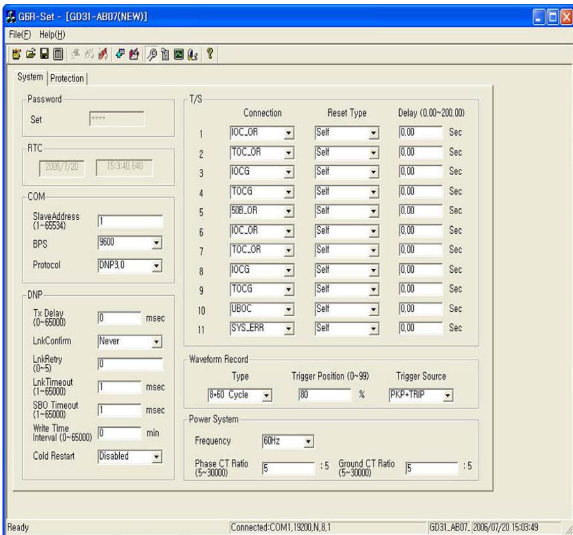
<Figure 14. GD31-AB07 System Configuration>
