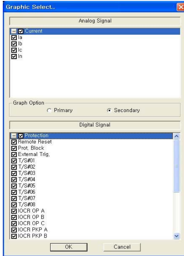
<Figure 20. GD31-AB07 Fault Evaluation Tool Graph>
