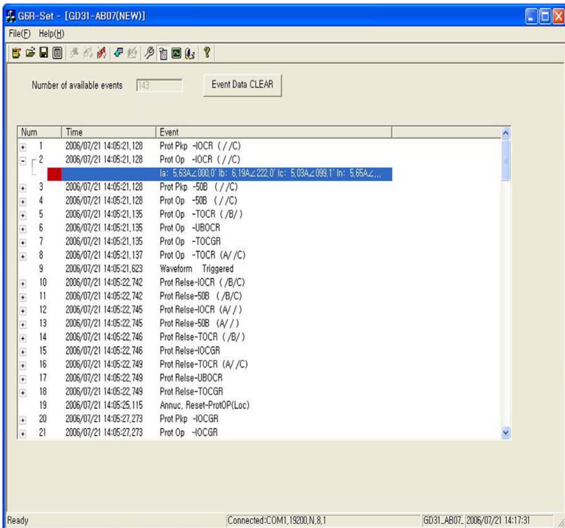
<Figure 16. GD31-AB07 Event>
