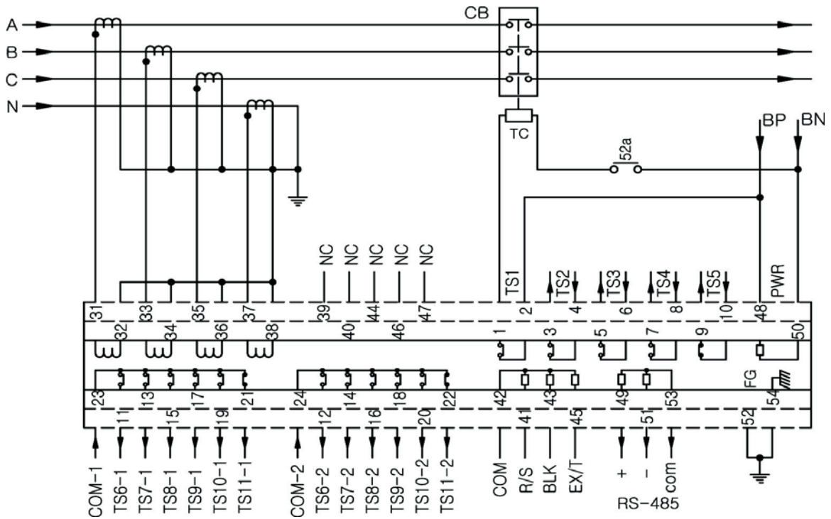
<부도 3. External Connection Diagram>
