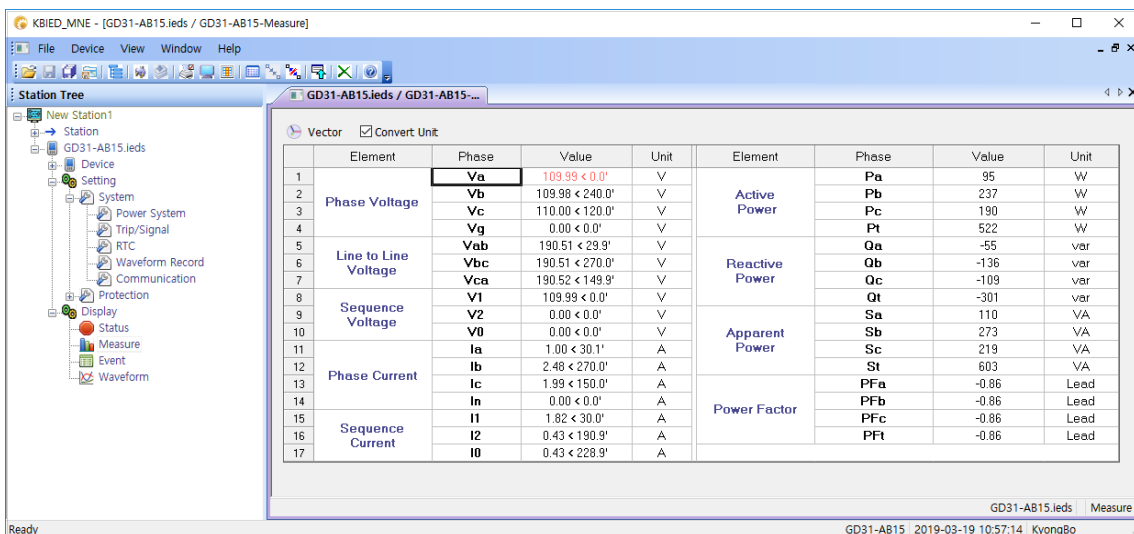
<Figure 30. Power Quantity>
