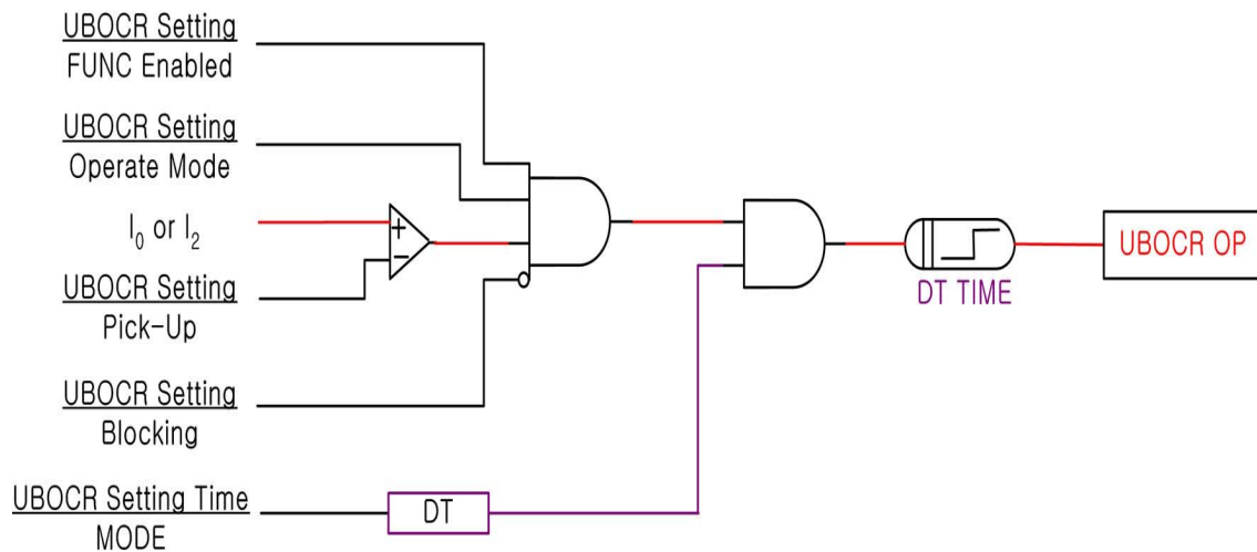
<Figure 6. UBOCR Logic Diagram>
