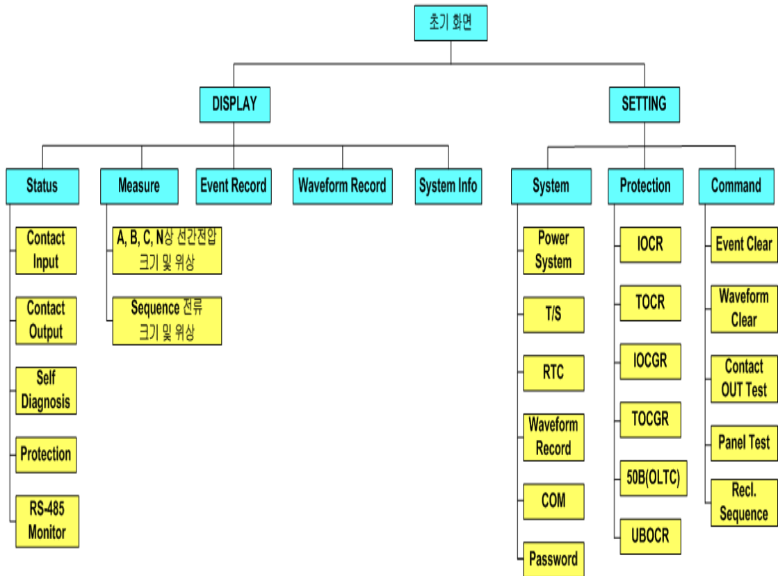
<Figure 11. Menu Tree>
