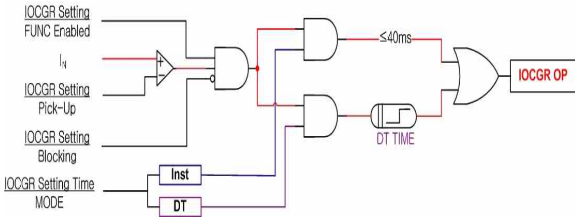
<Figure 3. IOCGR Logic Diagram>
