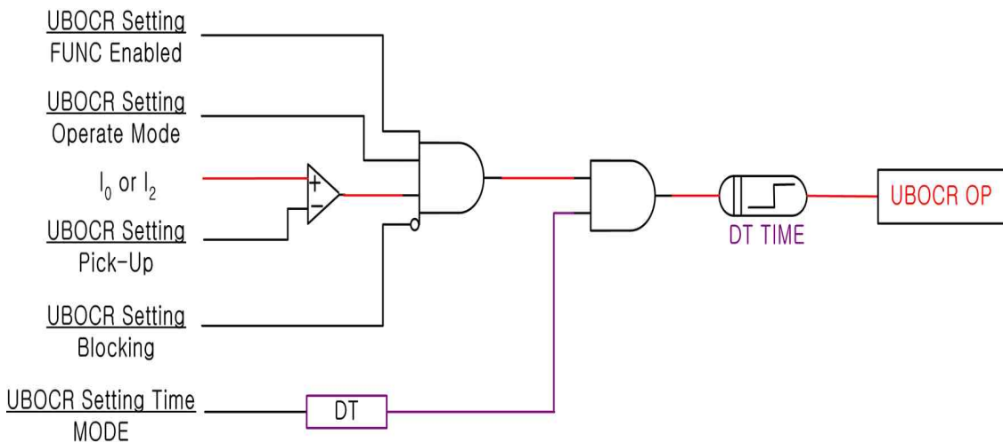
<Figure 6. UBOCR Logic Diagram>
