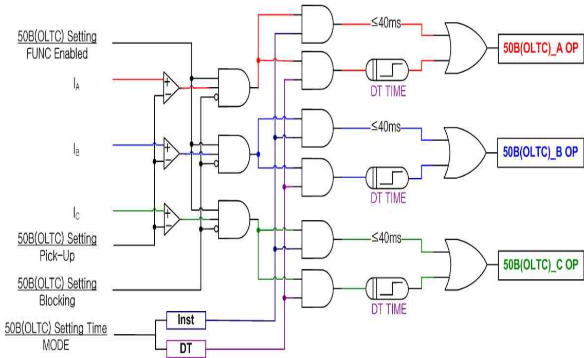
<Figure 5. 50B(OLTC) Logic Diagram>
