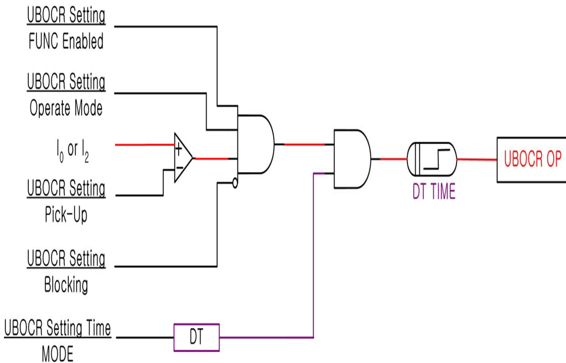
<Figure 6. UBOCR Logic Diagram>
