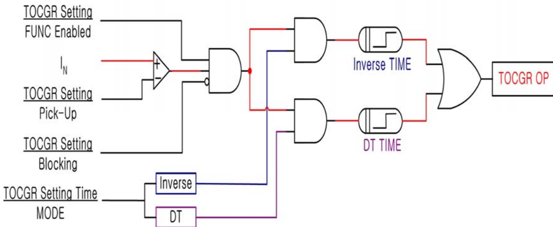
<Figure 4. TOCGR Logic Diagram>
