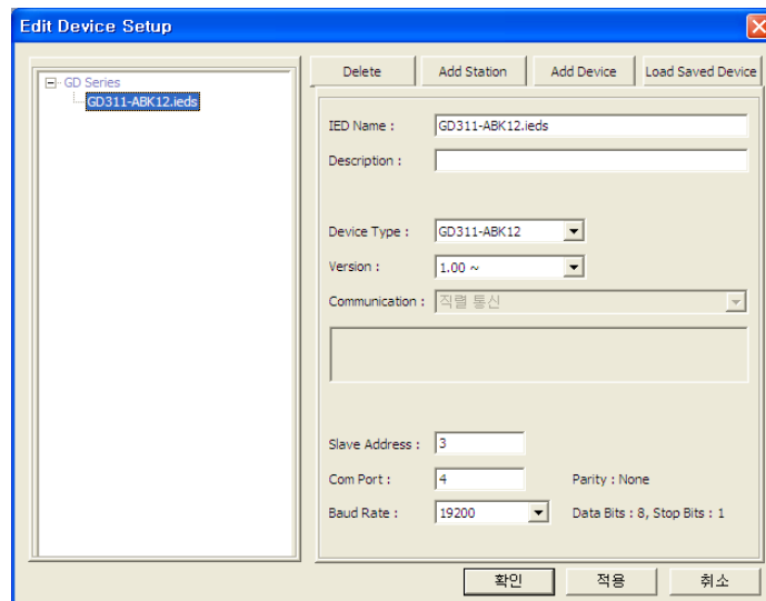
<Figure 16-2. Edit Devices - Device 화면>
