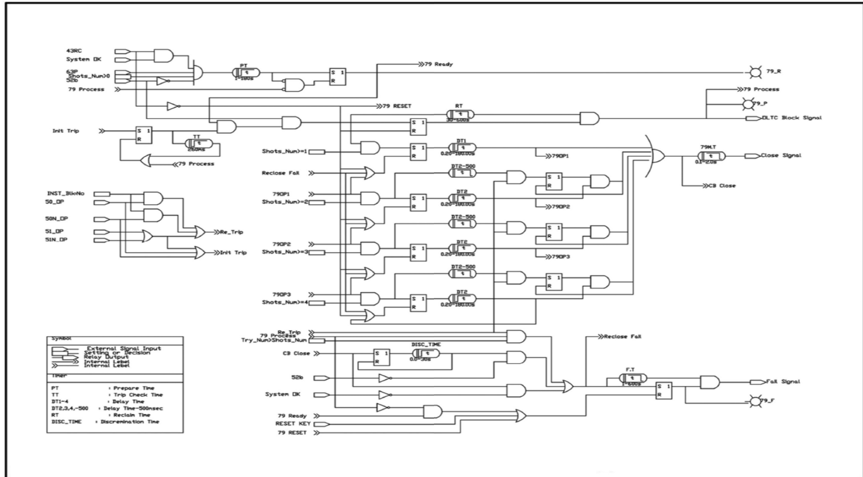
<Figure 7. Auto-Reclosing Logic Diagram>
