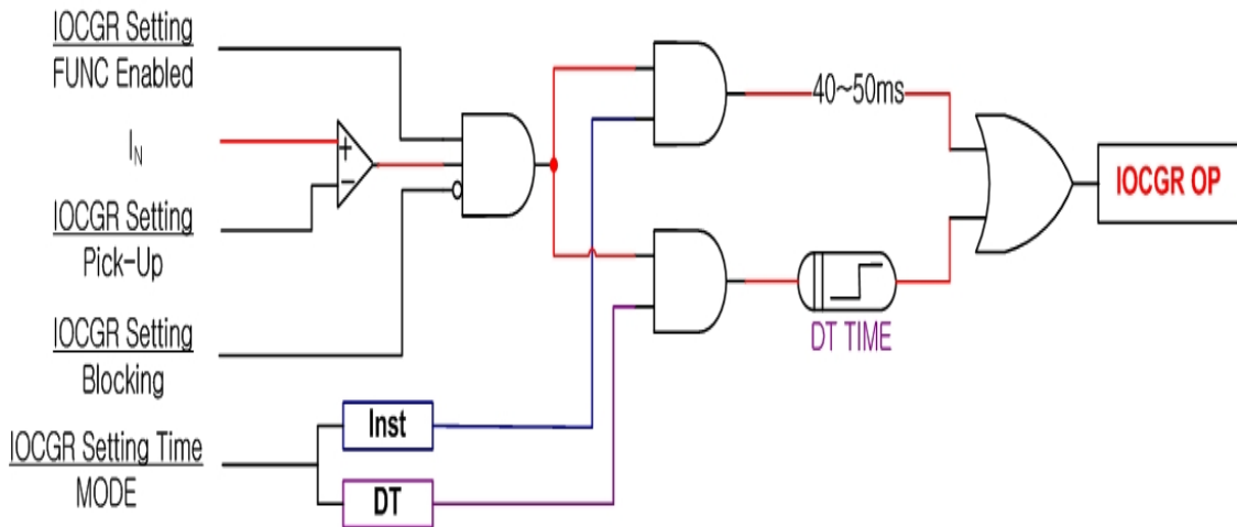
<Figure 3. IOCGR Logic Diagram>
