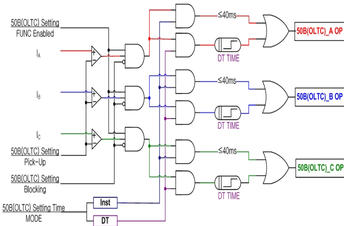
<Figure 5. 50B(OLTC) Logic Diagram>
