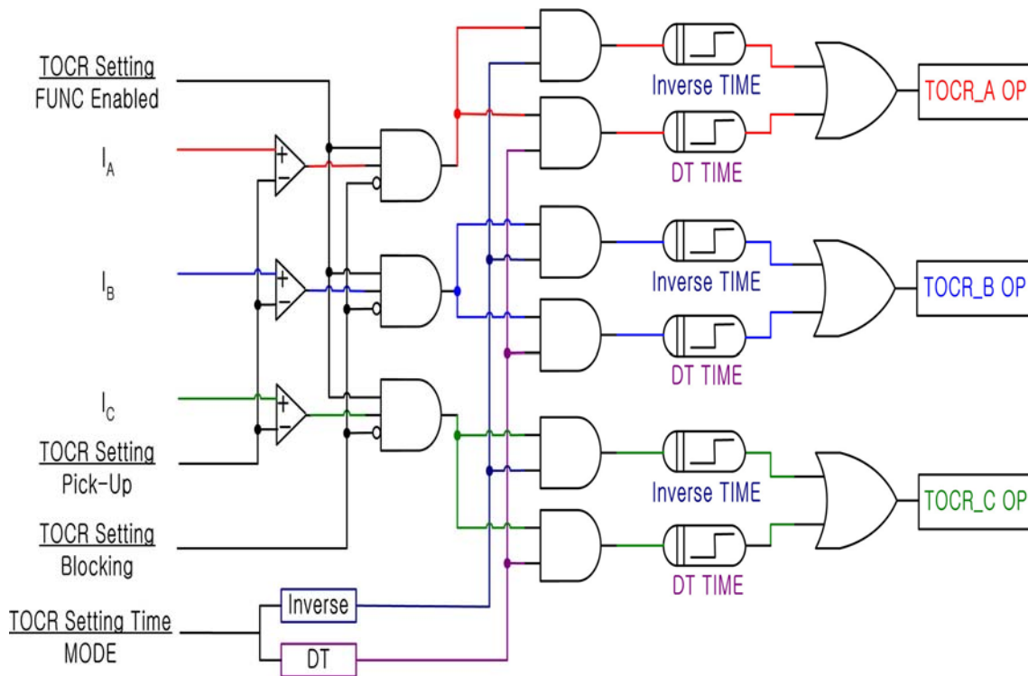
<Figure 2. TOCR Logic Diagram>
