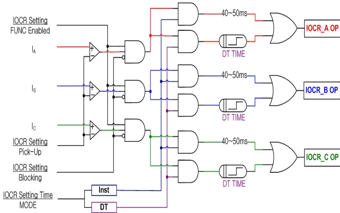
<Figure 1. IOCR Logic Diagram>
