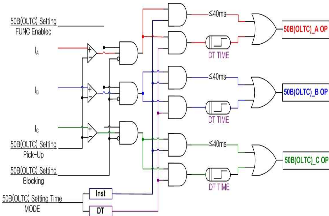
<Figure 10. 50B(OLTC) Logic Diagram>
