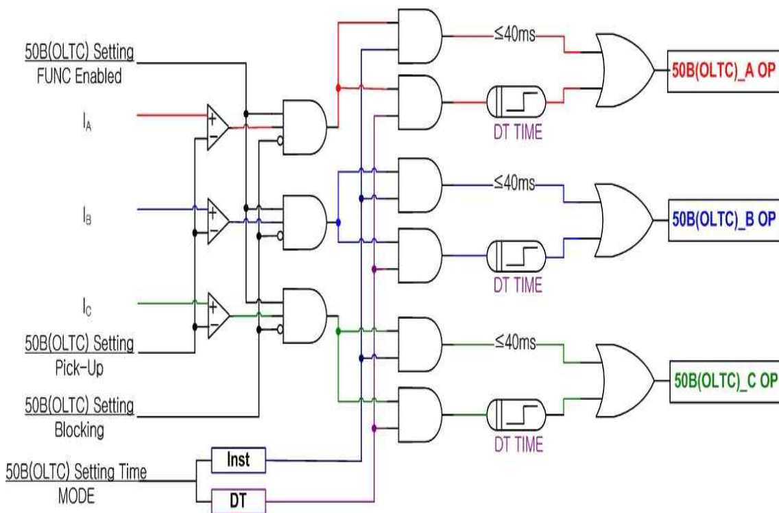
<Figure 10. 50B(OLTC) Logic Diagram>
