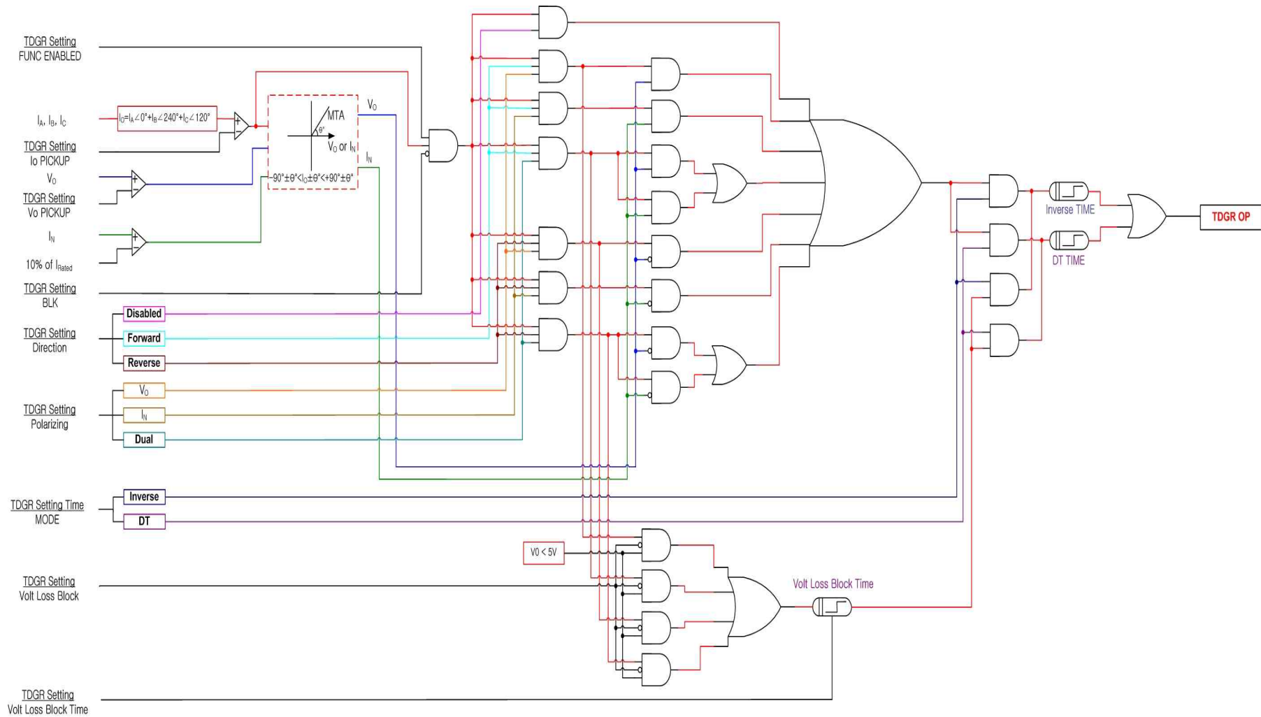
<Figure 8. TDGR Logic Diagram>
