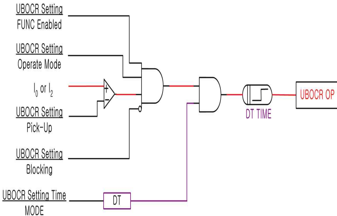
<Figure 11. UBOCR Logic Diagram>
