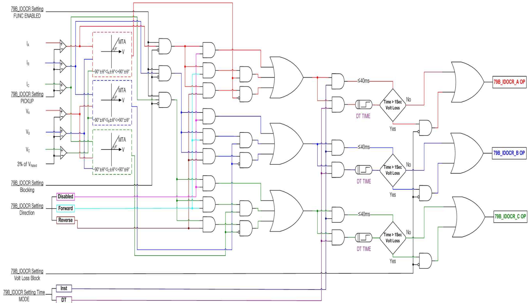
<Figure 5. 79B_IDOCR Logic Diagram>
