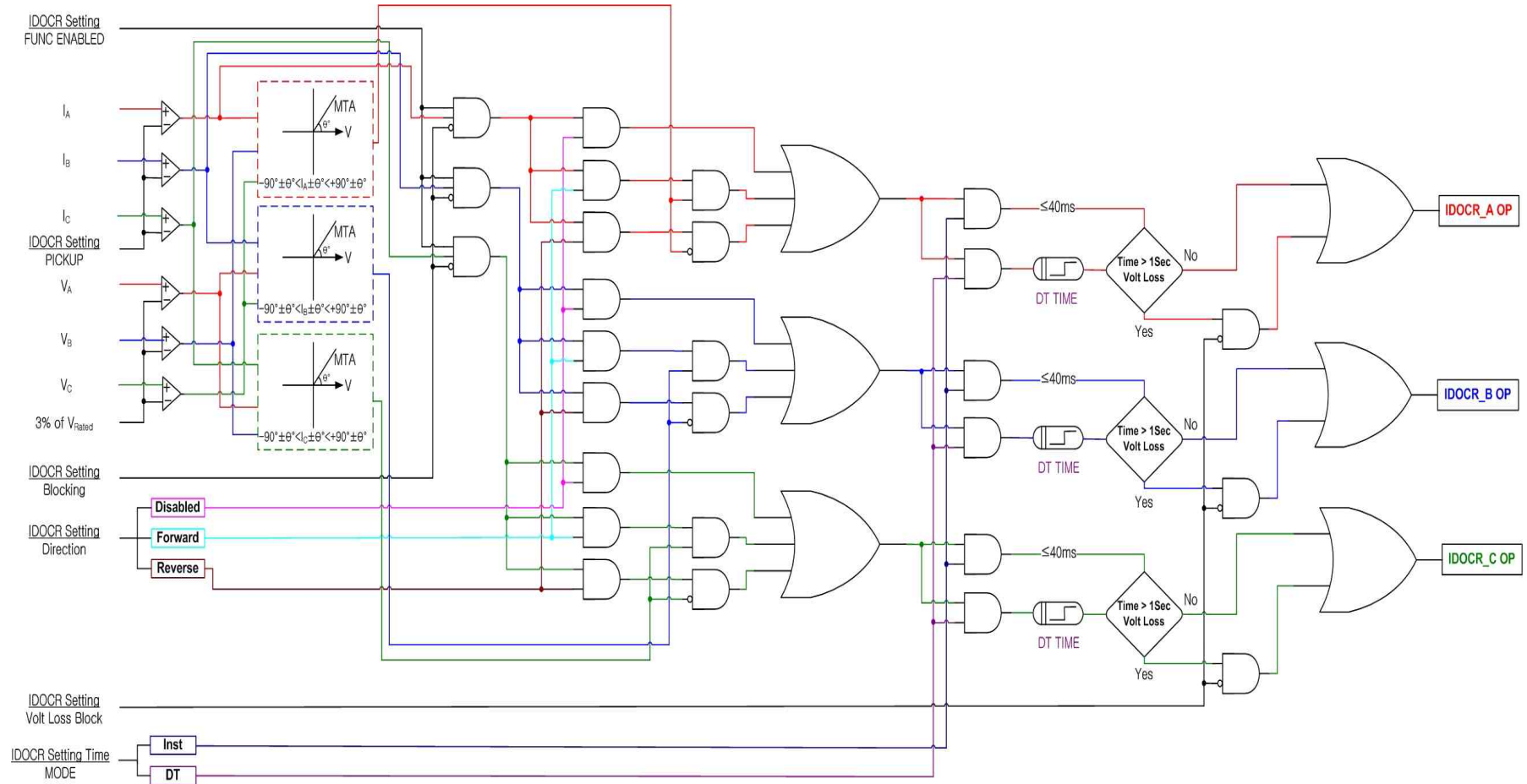
<Figure 3. IDOCR Logic Diagram>
