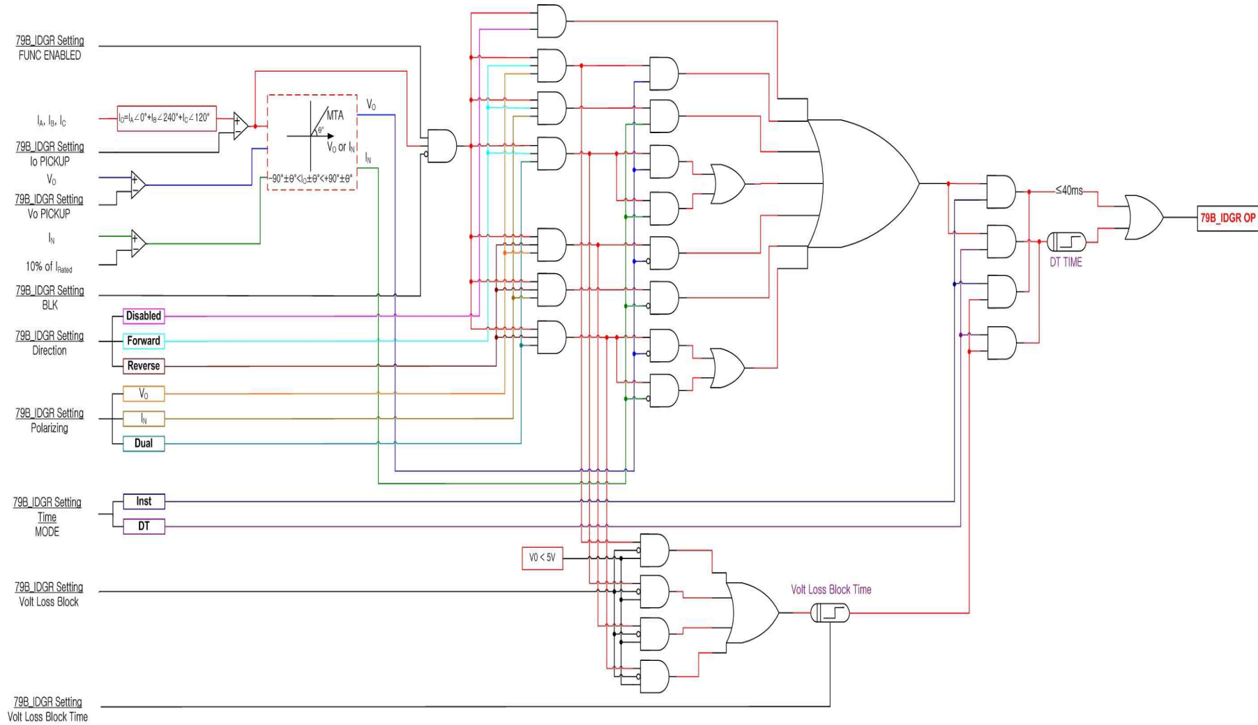
<Figure 9. 79B_IDGR Logic Diagram>
