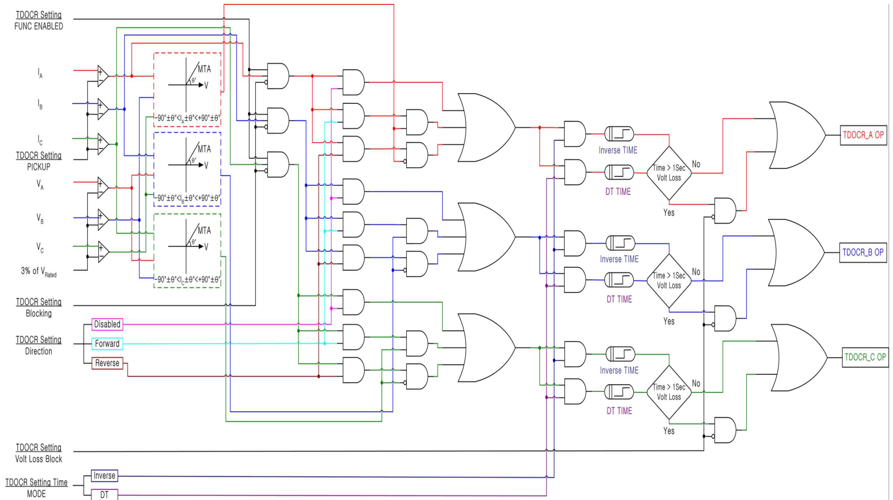
<Figure 4. TDOCR Logic Diagram>
