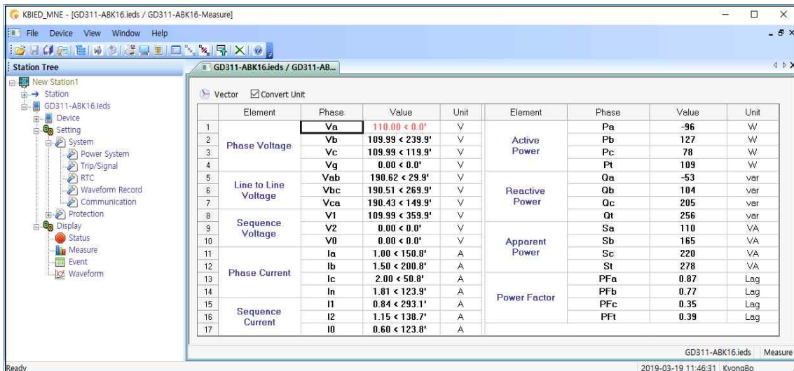
<Figure 35. Power Quantity>
