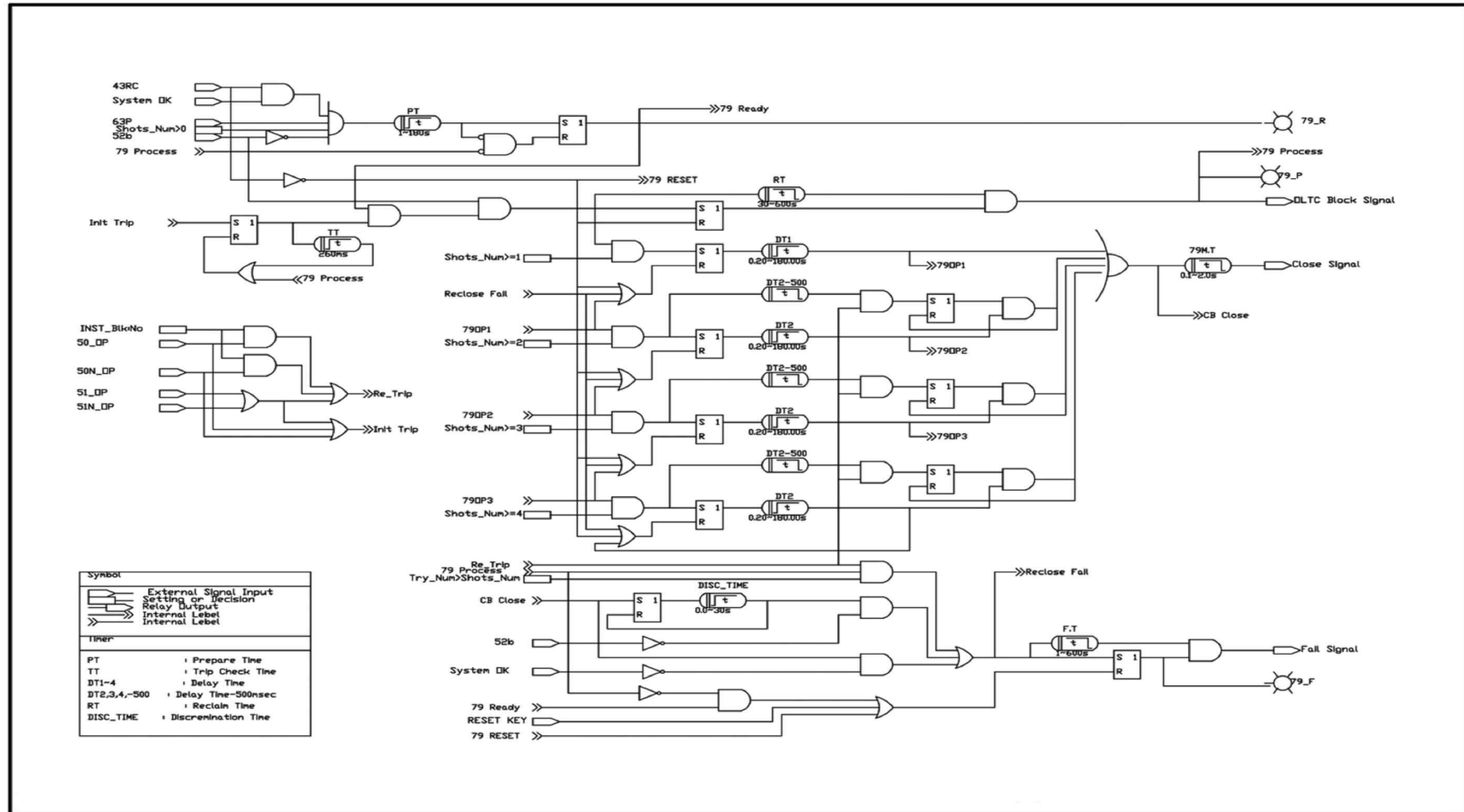
<Figure 12. Auto-Reclosing Logic Diagram>
