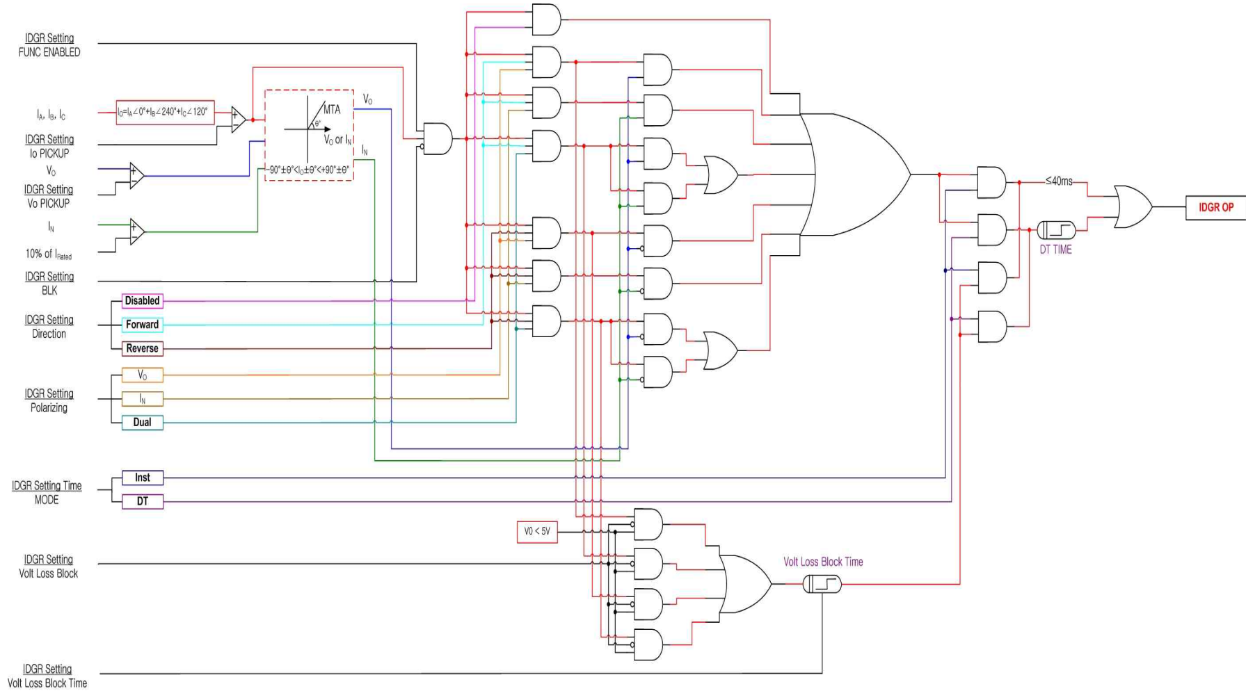
<Figure 7. IDGR Logic Diagram>
