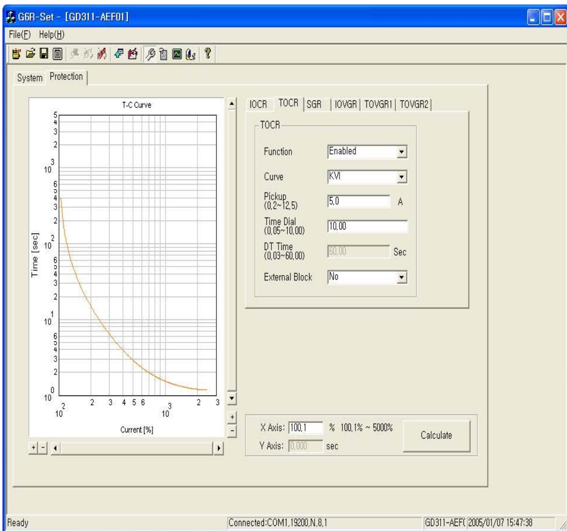
<Figure 17. GD311-AEF01 Protection Setting>
