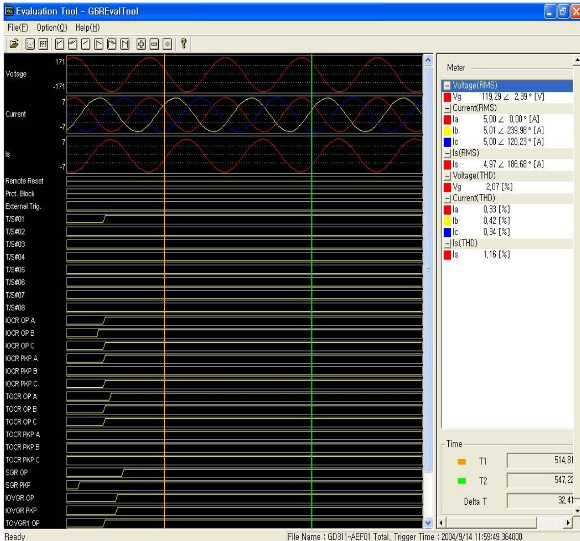
<Figure 21. GD311-AEF01 Fault Evaluation Tool>
