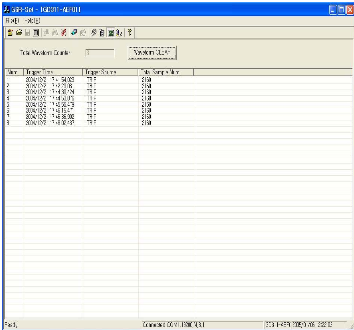
<Figure 19. GD311-AEF01 Waveform>
