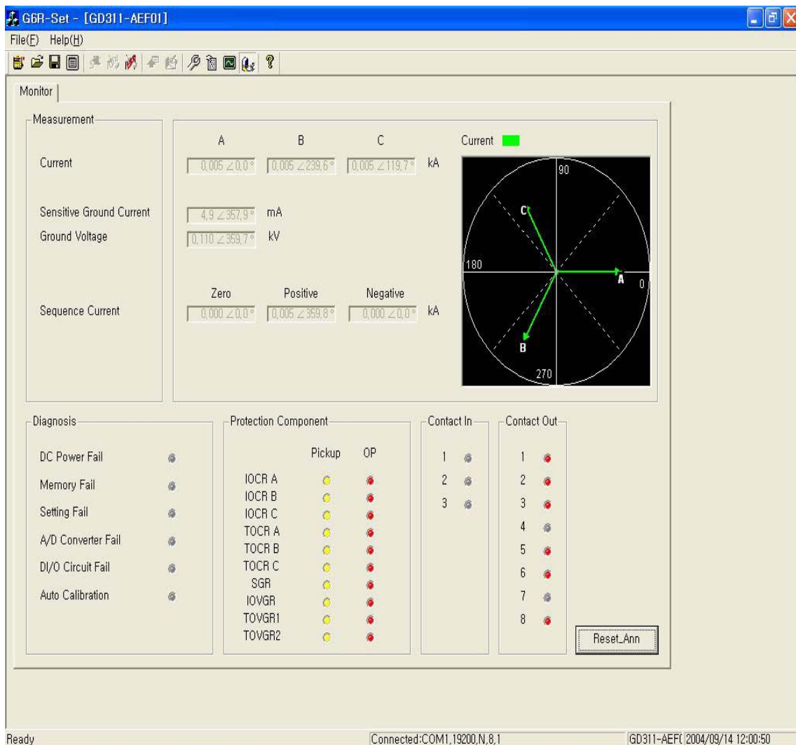
<Figure 20. GD311-AEF01 Monitor>
