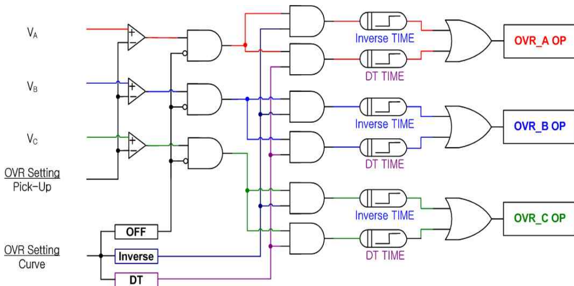
[Figure 3.1] OVR Logic Diagram
