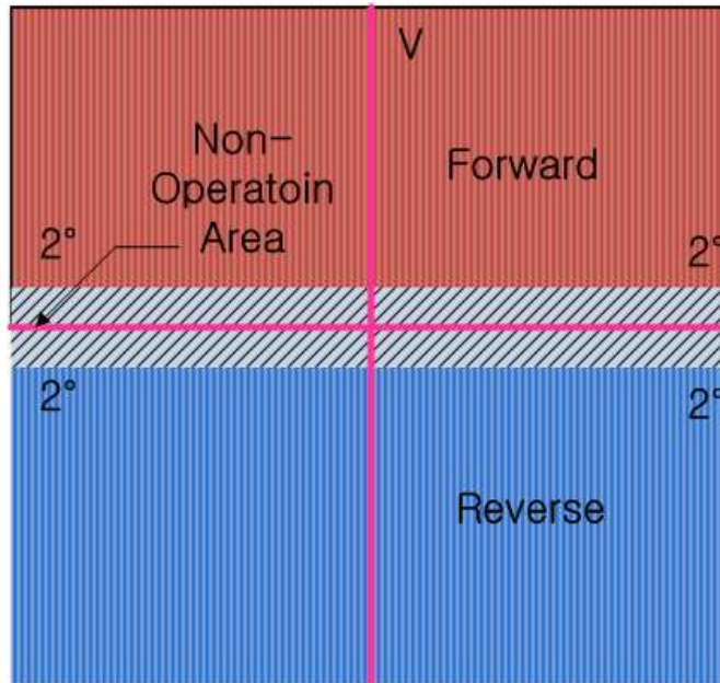
【Figure 3.3】 UPR Directional operation characteristic
