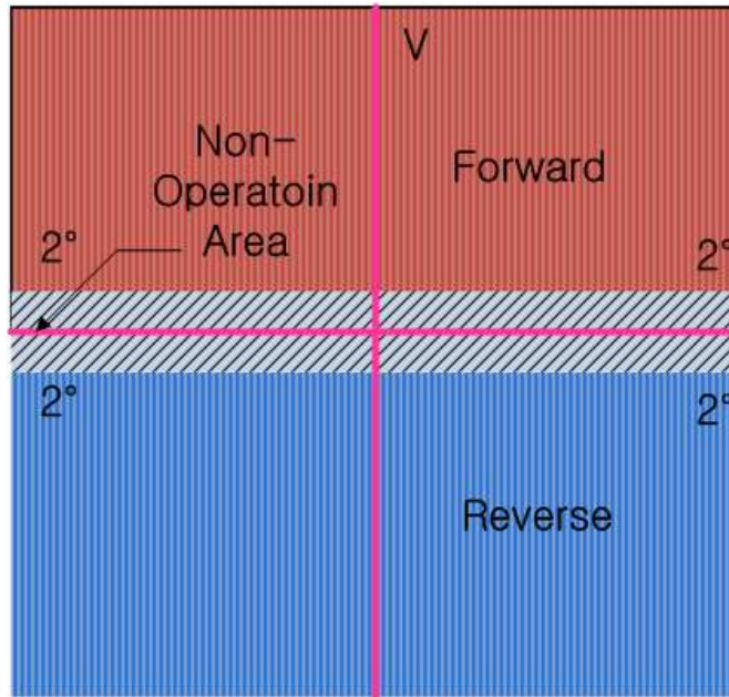
【Figure 3.1】 O(R)PR Directional operation characteristic
