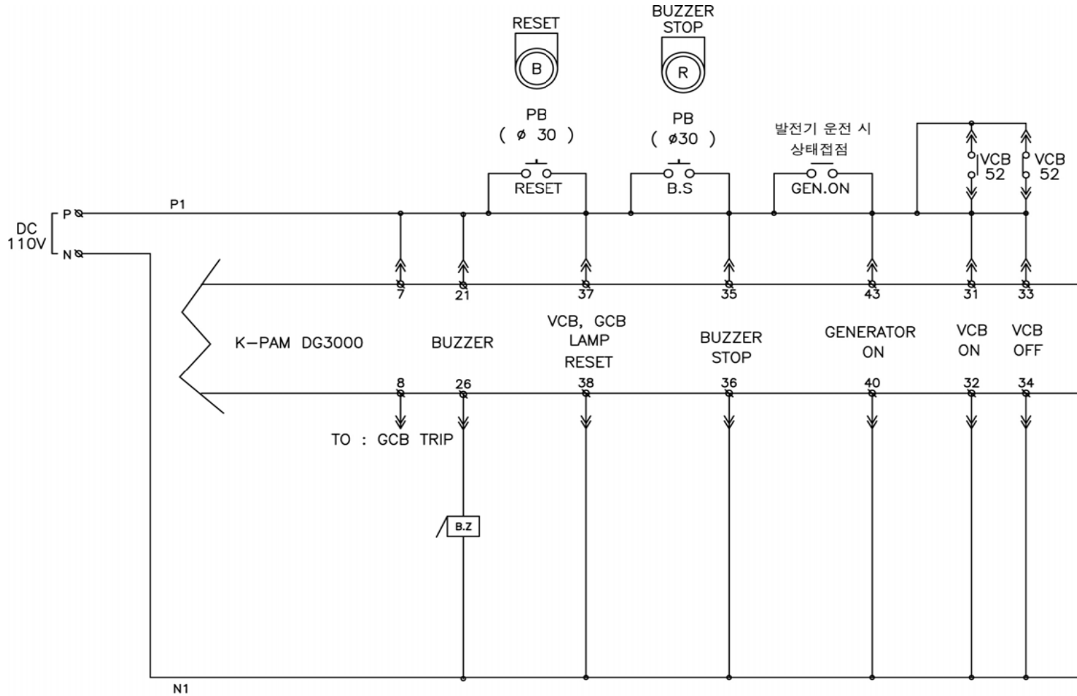
GCB & Buzzer, Digital Input DC SEQUENCE DIAGRAM
