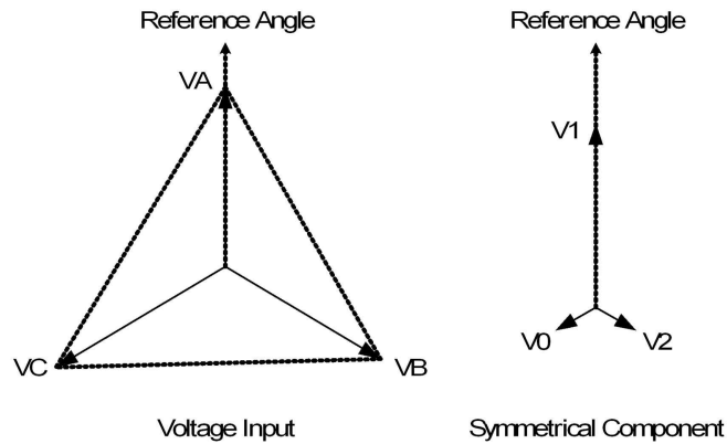
<Figure 94. Sequence 전압>
