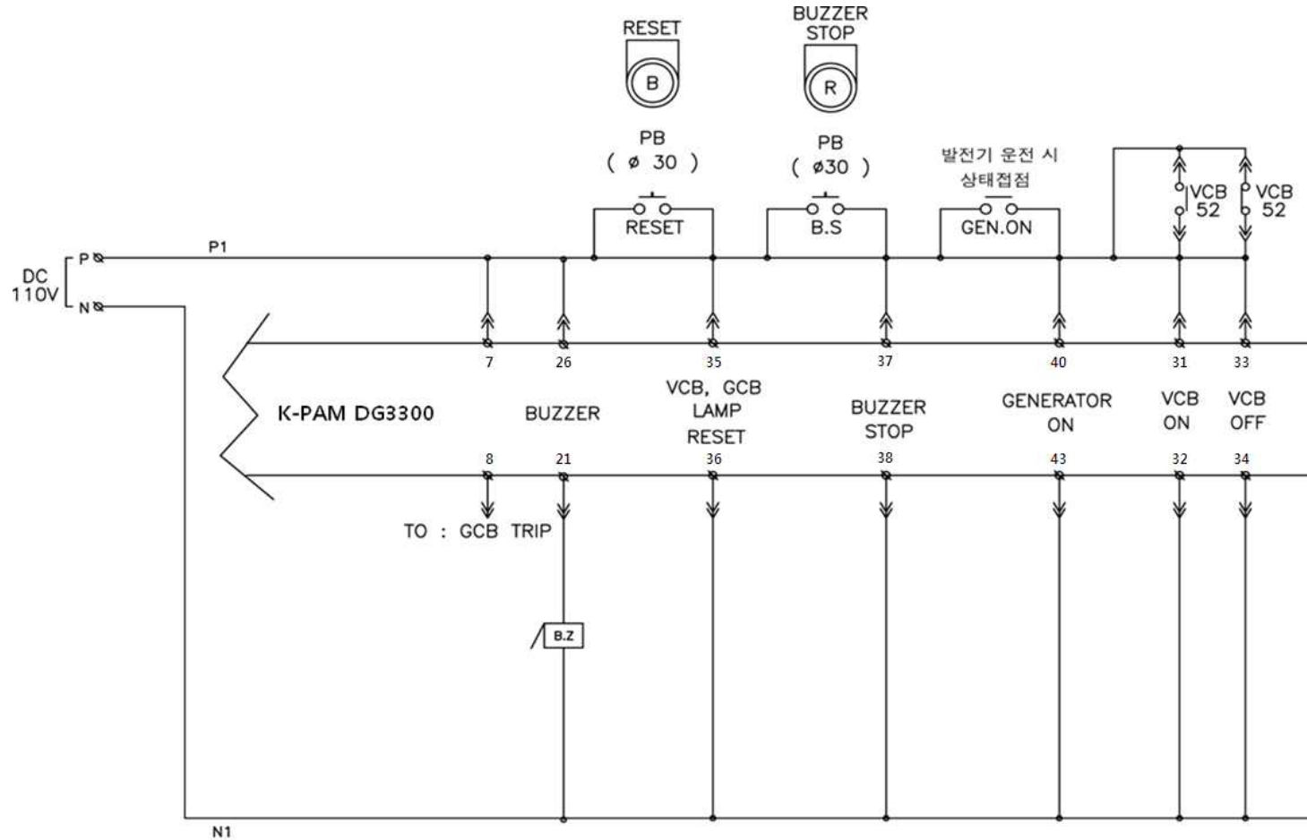
GCB & Buzzer, Digital Input DC SEQUENCE DIAGRAM
