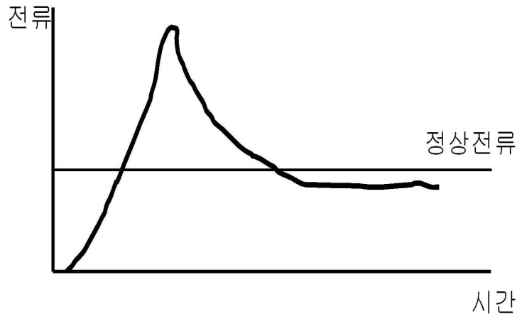
<Figure 44. Cold Load Pickup 전류 형태>
