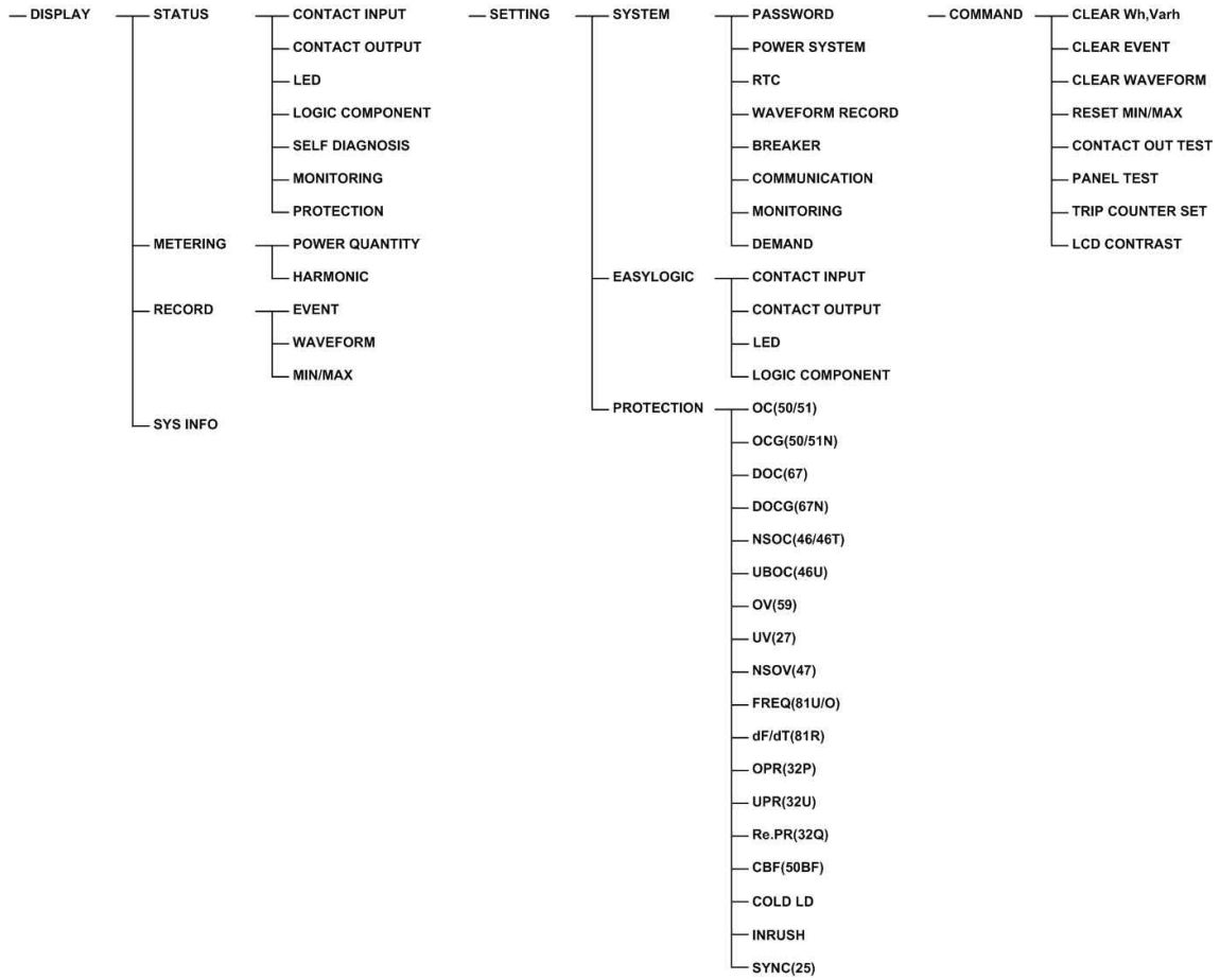
<Figure 4. DG3300 Menu Tree>
