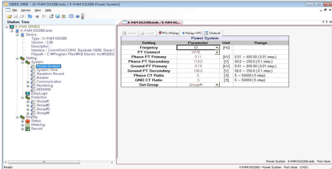
<Figure 63. Power System 화면>
