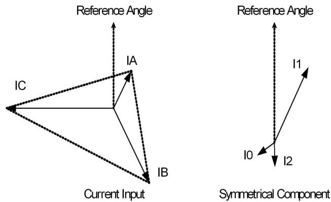
<Figure 95. Sequence 전류>
