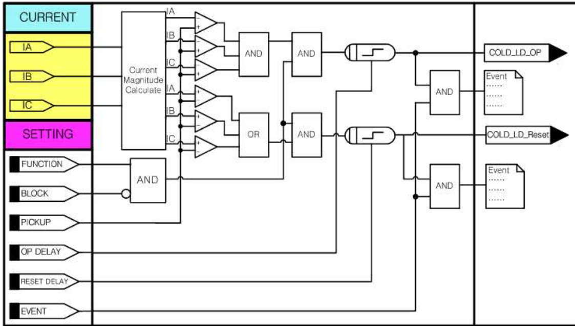
<Figure 45. Cold Load Pickup 동작특성>
