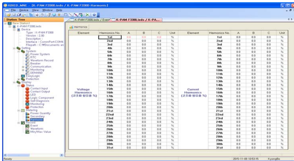
<Figure 82. Harmonic>
