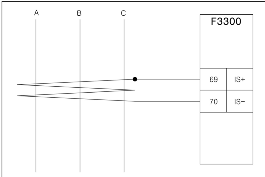
<Figure 101. ZCT 결선>
