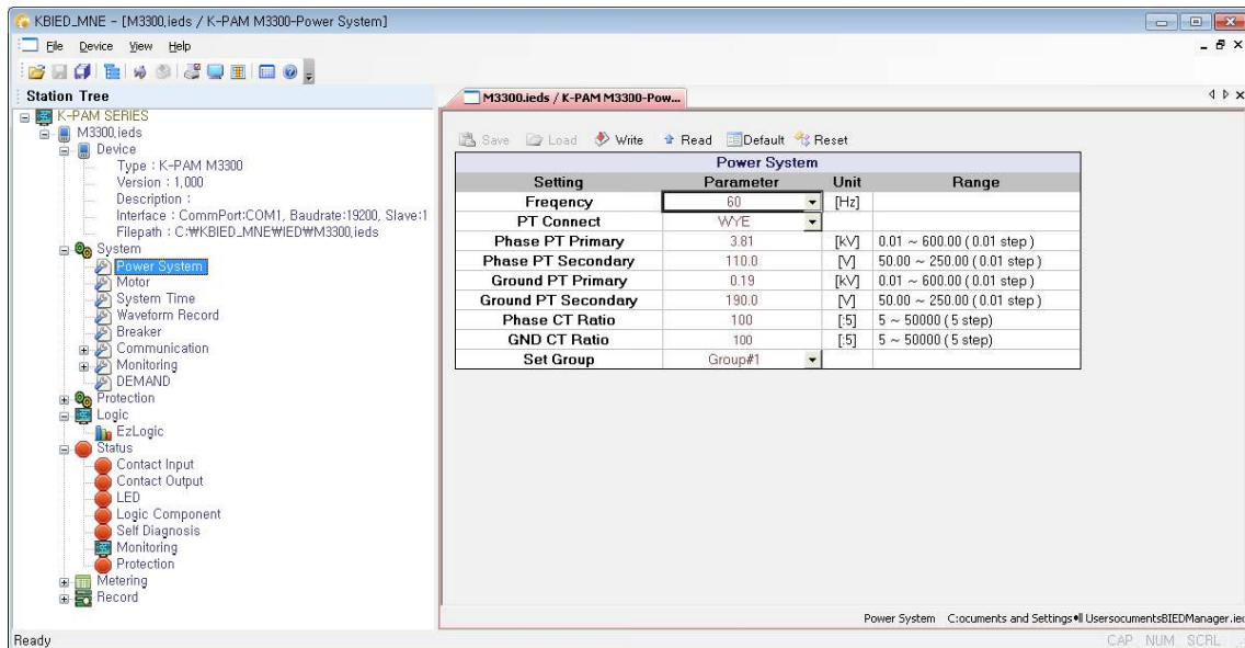
<Figure 60. Power System 화면>
