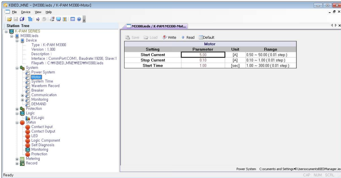
<Figure 61. Power System 화면>
