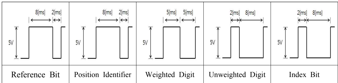
<Figure. IRIG-B00X Bit Pulse Width>
