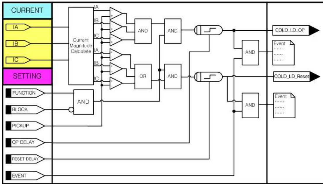
<Figure. Cold Load Pickup 동작특성>
