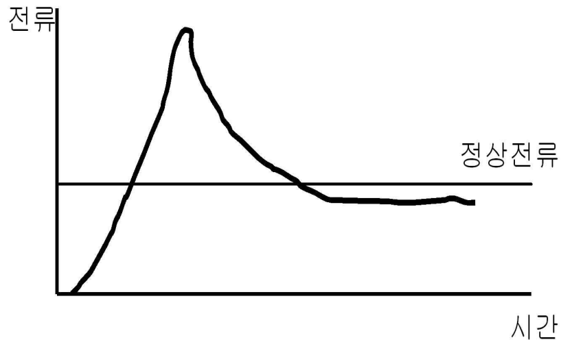
<Figure. Cold Load Pickup 전류 형태>
